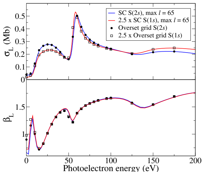
FIG. 11. Comparison between the photoionization of SF_6 from the S(1s) and S(2s) orbitals, for the cross section (top) and \beta parameter (bottom). The cross section corresponding to the S(1s) photoionization has been resized by a factor of 2.5 to compare better the energy dependence.
