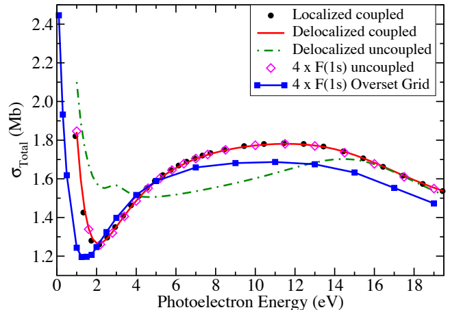
FIG. 6. Total cross sections for F K-edge photoionization in \text{CF}_4 from basis-set Kohn calculations in the length gauge summed over the four channels. Curves labeled delocalized have channels defined as vacancies in the four orbitals of a_1 and t_2 symmetry in tetrahedral symmetry. Curves labeled “localized” have one channel defined as a F(1s) vacancy and the other three as vacancies in the remaining a_1 and e symmetry in C_{3v} symmetry. The curves labeled “F(1s)” are four times the cross section for a single channel defined as a vacancy in one fluorine 1s orbital. The overset-grid result for the F(1s) channel is also shown.
