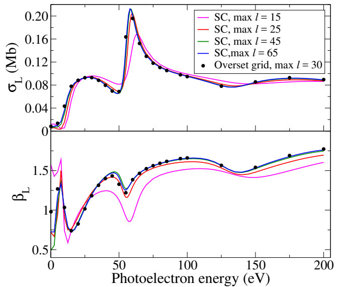
FIG. 10. Photoionization cross section (top) and \beta parameter (bottom) of SF 6 from the S(1s) orbital, computed with the single center expansion for different values of the maximum angular momentum \ell and the converged overset-grid result.
