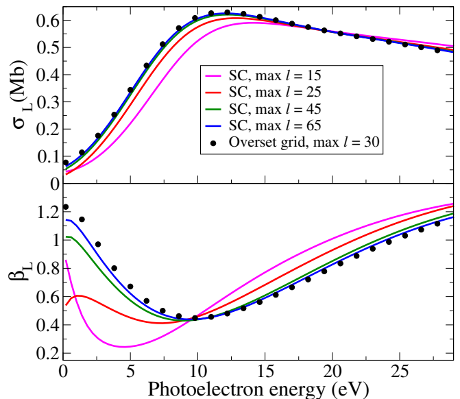
FIG. 2. Integral cross section (top) and \beta parameter (bottom) for the angular distribution of the photoelectron relative to polarization direction for ionization of the carbon 1s orbital in CF_4 , comparing the converged oversight-grid results with those using a single center expansion and the Schwinger iterative method.
