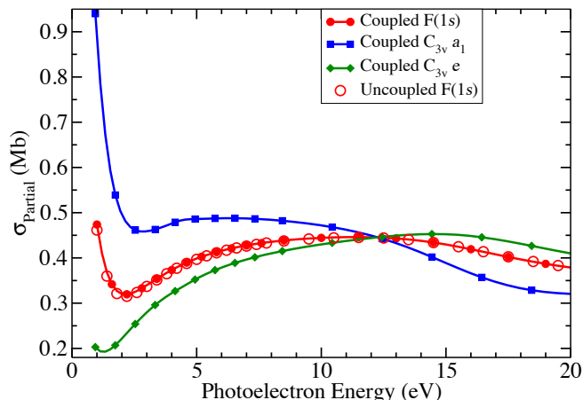
FIG. 8. Partial photoionization cross sections for each of the four channels from coupled-channel basis-set Kohn calculations with one channel defined as a F(1s) vacancy and the other three as vacancies in the remaining C 3v symmetry orbitals. The cross sections from the two different e symmetry orbitals are the same. The single-channel (uncoupled) results for the F(1s) hole are shown as symbols alone, and are seen to be nearly identical to the F(1s) coupled channel results.
