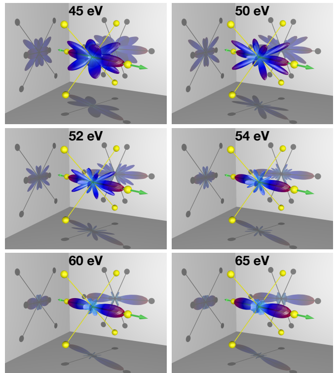
FIG. 12. Calculated MFPADs corresponding to different photoelectron energies (shown in the insets), for the SF_6 photoionization from the S(2s) orbital, with a linearly polarized field along one of the main molecule axis.
