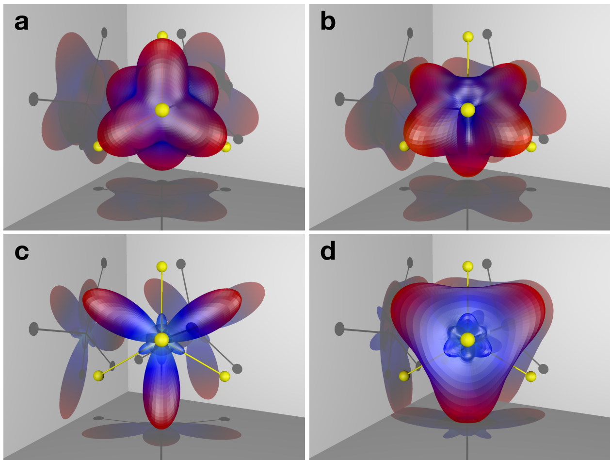
FIG. 9. Calculated PA-MFPADs from delocalized and localized hole states for ionization from the F K-edge in \text{CF}_4 2 eV above threshold. (a) The total PA-MFPAD summed over all four channels ( a_1 and t_2 orbitals) in tetrahedral symmetry coupling the four channels using delocalized hole states; (b) The same calculation using delocalized hole states with the four channels uncoupled, showing broken symmetry from the single-channel treatment; (c) The same calculation (from the overset-grid implementation) in the full T_d symmetry using delocalized hole states, recovering the symmetry but not the correct coupled channel result, and (d) The PA-MFPAD (times 2.75) for ionization of the localized F(1s) hole on the F atom pointing towards the viewer from the single-channel calculation, which when rotated on to the other three CF directions and summed reproduces (a).
