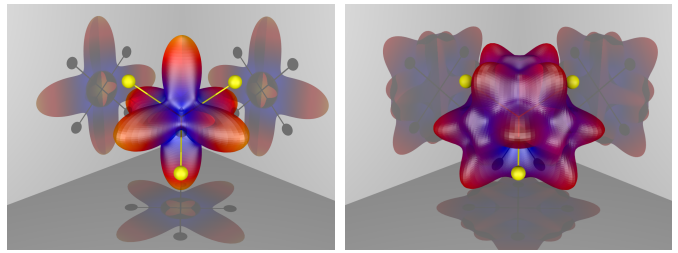
FIG. 4. PA-MFPADs for carbon 1s ionization at 4 eV (left) and 13 eV (right scaled by 2.3). The “anti imaging” angular dependence on the left is essentially identical to the basis-set Kohn result in Fig. 5 of ref. [8] where it is compared with experiment.
