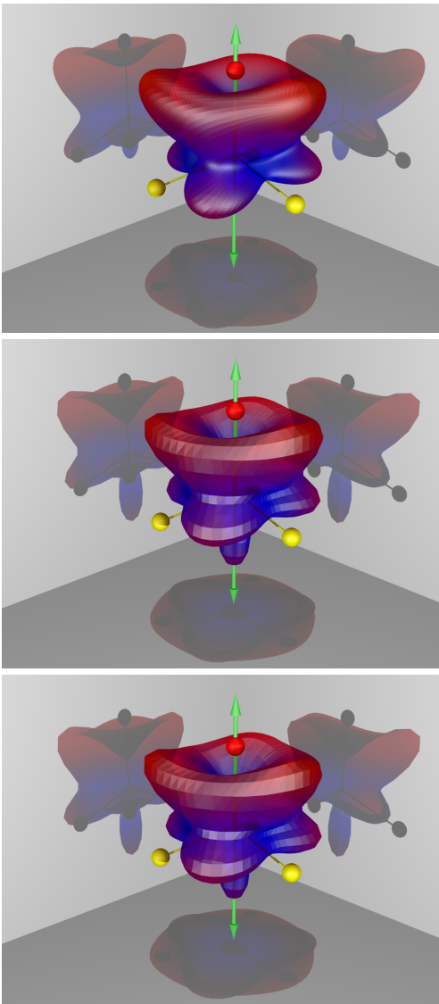
FIG. 5. MFPADs for a 3 eV photoelectron from ionization by linear polarization along a CF bond (two-headed green arrow) for the creation of F(1s) hole localized on the F atom on the polarization axis, which is shown in red. All three calculations used the localized orbitals with one orbital corresponding to the localized F(1s) hole state and the other three F(1s) orbitals being delocalized on the other F atoms. The top panel shows the results from the single-channel overset-grid calculation. The middle panel shows the results from the single-channel basis-set Kohn calculation. And the bottom panel shows the basis-set Kohn results with all four F(1s) ionization channels coupled.
