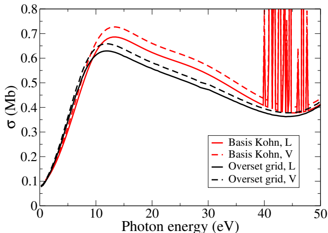
FIG. 3. Integral cross section for C(1s) ionization in CF_4 comparing basis-set Kohn variational calculations in both length (L) and velocity (V) gauges with converged overset-grid results. The breakdown seen in the basis-set Kohn calculations at energies above 40 eV is due to the limited basis set used in the expansion in Eq. (4)
