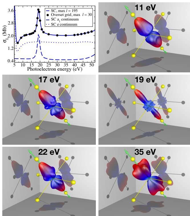
FIG. 13. Total MFPADs corresponding to a fixed polarization direction along the principal molecular axis, for several photoelectron energies (shown in insets) around the shape resonance peak displayed on the top-left panel, obtained adding up the 6 \text{SF}_6 photoionization channels that leave the parent ion with a localized 1s hole on each fluorine atom.
