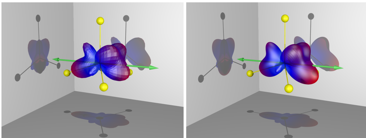
FIG. 7. Comparison of calculated MFPADs for F(1s) ionization of CF 4 by linearly polarized light, with the polarization direction indicated by the two headed green arrows. On the left, the results of a basis-set complex Kohn method at its Cooper minimum (2.18 eV), from a coupled four channel calculation with the MFPAD summed over all four channels. On the right, a single channel overset-grid calculation at its Cooper minimum (1.5 eV), where the F(1s) hole is localized on one F atom and the MFPAD is summed over four such single-channel calculations with the F(1s) hole being localized on the different F atoms.
