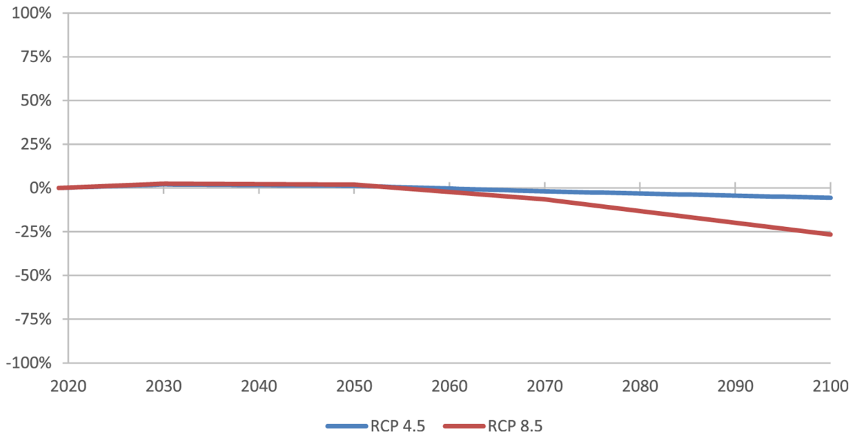
Figure 2. Projected changes in thermally available habitat, American lobster, East Coast: Five-GCM mean.
