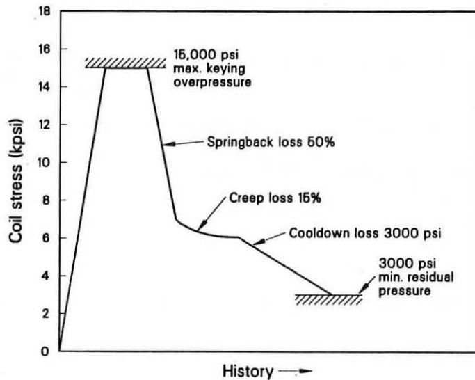
Fig. 4. Coil Stress History with Stress Limits
