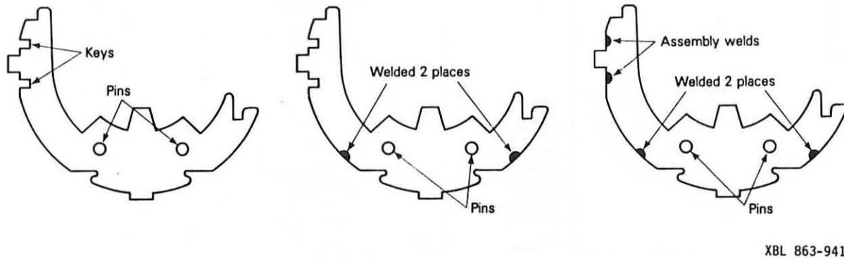
Fig. 5. Modified Keyed Fig. 6. Partially Welded (welds supplement pins only) Fig. 7. Fully Welded (No Keys)
