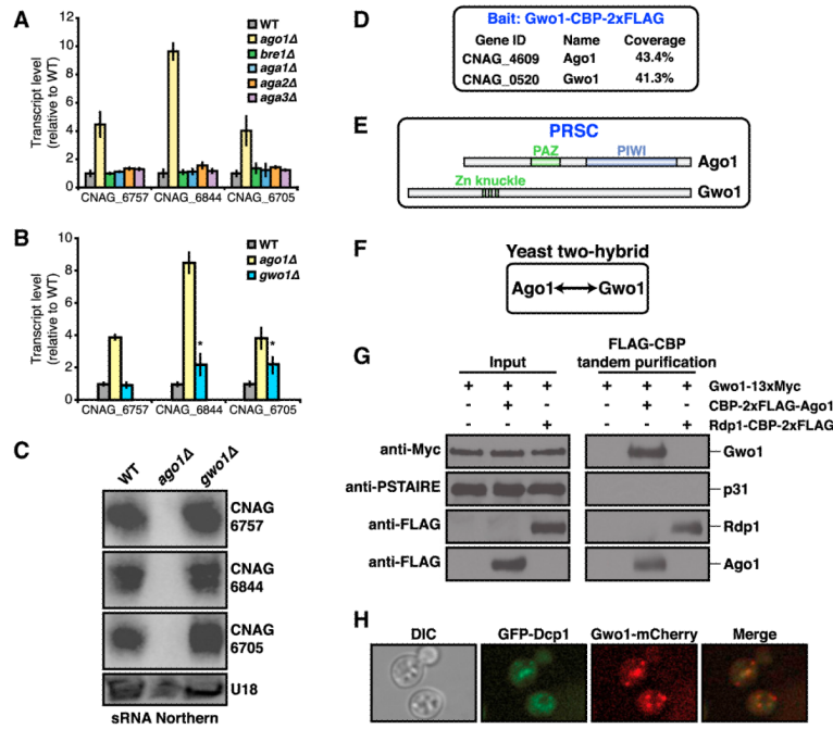
Figure 3. PRSC and SCANR Subunits Are Physically and Functionally Distinct (A and B) Transcript levels of three RNAi target genes, assessed by RT-qPCR and normalized to 18S rRNA levels. Error bars represent SEM. * p < 0.05 by Student's t test. (C) sRNA Northern blot. Loading control: U18 snoRNA. (D) Proteins associated with Gwo1-CBP-2xFLAG. Assayed as in Figure 2A. (E) Predicted protein domains of PRSC subunits. (F) Protein-protein interactions among PRSC components, as assessed by yeast two-hybrid assay. No interactions were detected between Gwo1 and any exclusive member of SCANR. (G) Coimmunoprecipitation of Gwo1 with Ago1, but not with Rdp1. Strains expressing Gwo1-13xMyc and CBP-2xFLAG-Ago1 or Rdp1-CBP-2xFLAG were subjected to FLAG-CBP tandem purification. Input and purified material were analyzed by immunoblot using anti-FLAG, anti-Myc, or anti-PSTAIRE, which detects the negative control protein p31. (H) Colocalization of PRSC component Gwo1 with the P body marker Dcp1. Unfixed cells were examined after incubation in yeast nitrogen base (YNB) media. See also Figure S1 and Table S3.
