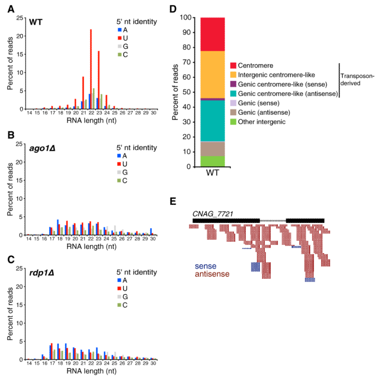
Figure 1. Endogenous siRNA of C. neoformans
