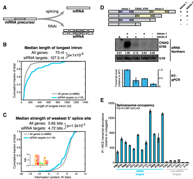
Figure 5. Transcripts Targeted by RNAi Display Suboptimal Splicing Features and Are Stalled on Spliceosomes In Vivo
