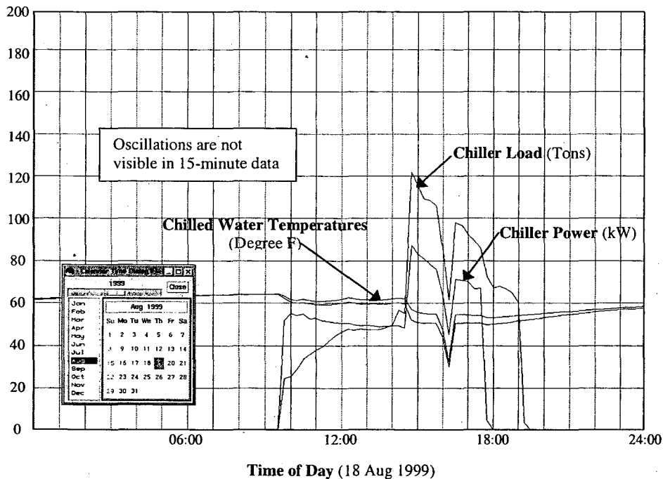
Figure 2-4 Oscillations not apparent using 15-minute data.
