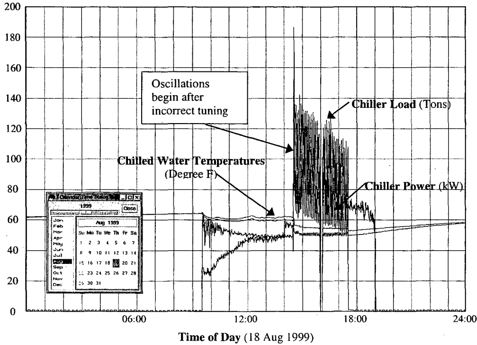
Figure 2-3. Oscillations viewed with 1-minute data.
