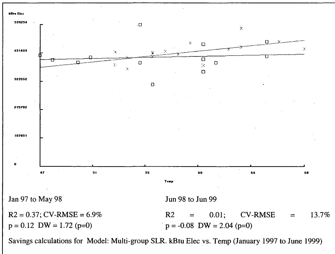
Figure 5-1. Monthly electricity (kBtu) versus average outside temperature (degree F).
