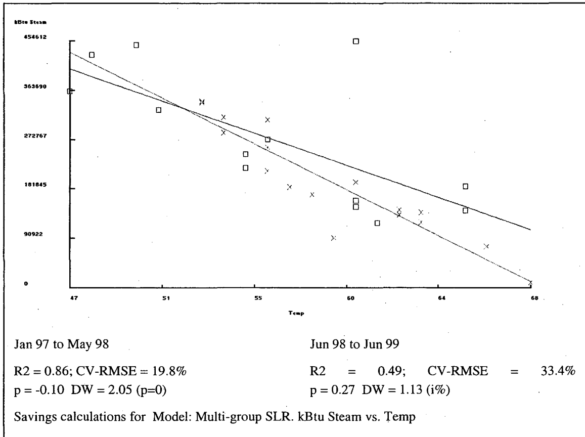
Figure 5-2. Monthly steam (kBtu) versus average outside temperature (degree F).
