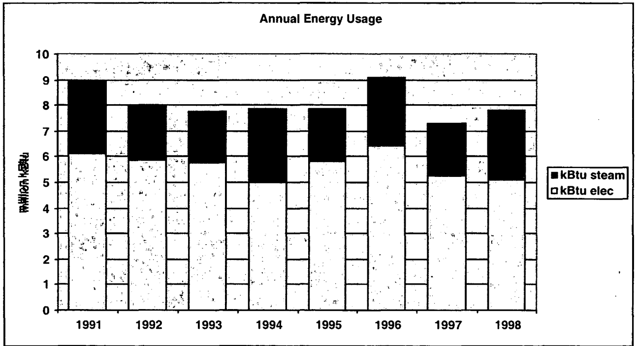
Figure 5-4. Multi-year whole-building energy use.
