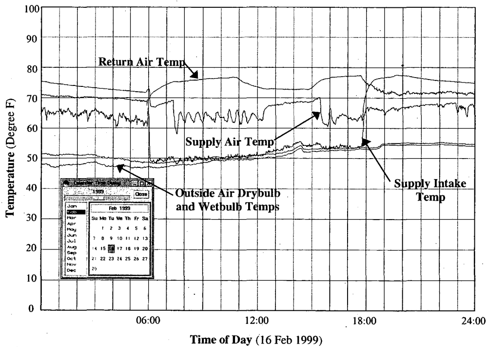
Figure 2-2. Supply air temperature with good control.
