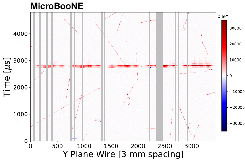
Figure 25: Example of an event in MicroBooNE data that is impacted by the purity-monitor-induced burst noise issue. Shown is an event display for the waveform data associated with Y plane wires after coherent noise filtering is carried out in units of electrons per 3 \mu s. Noisy and unresponsive channels are shaded grey in this illustration. One distinctive feature of the purity-monitor-induced burst noise is a strong isochronous signal across all wires that is most severe on the Y plane (as seen by the horizontal band in the display). Another feature of this specific type of burst noise is the large amount of light observed in the PMTs in the same event (discussed later). The noise feature is not removed from data by the coherent noise filtering procedure that is applied to raw data.
