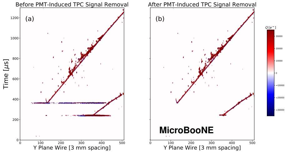
Figure 21: Event display of the collection plane (Y plane) before (a) and after (b) removal of PMT pick-up noise, after carrying out the deconvolution in both cases in units of electrons per 3 \mu\text{s} . The event display is zoomed-in to a small part of the detector where PMT-induced TPC signals are observed in the event. The horizontal blue and red streaks seen in the bottom of the left image, which are attributed to capacitive-coupling between a PMT and the TPC wires, are largely removed via a dedicated algorithm.
