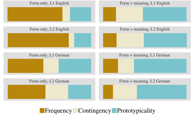
Figure 3: Contributions of the predictors across the analyses.
