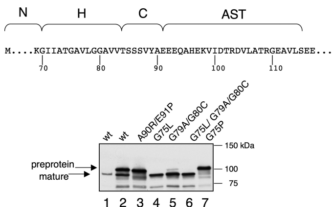
FIGURE 2. Accessory Sec-independent transport of GspB 736FLAG and selected variants in E. coli . The amino acid sequence of the H and C regions of the signal peptide, along with the AST domain of GspB is indicated. The GspB 736FLAG variants were expressed constitutively from pVA891 (26, 27), and were detected by Western blotting with anti-FLAG monoclonal antibodies. Lane 1, periplasmic proteins; lanes 2–8, whole-cell lysates.
