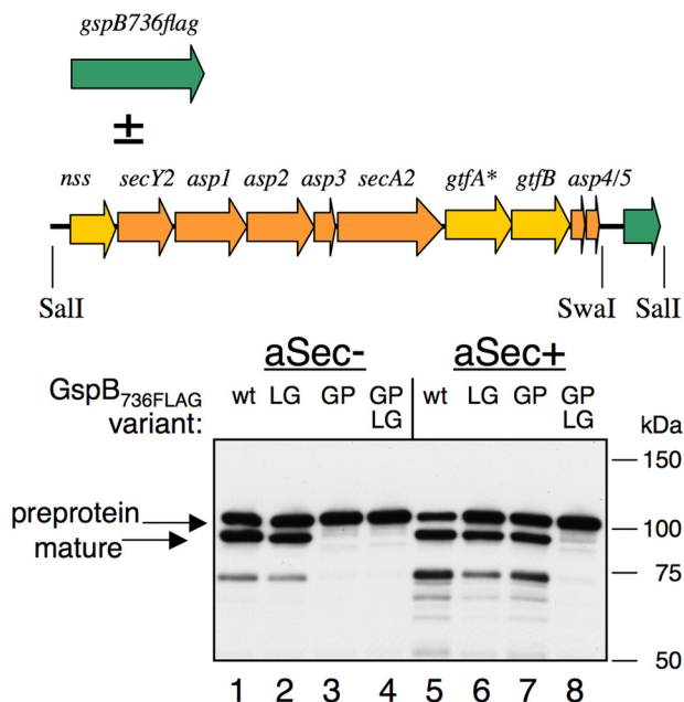
FIGURE 3. Transport of GspB 736FLAG and selected variants in the absence or presence of the aSec system in E. coli (aSec - , or aSec + , respectively). GspB 736FLAG (wt) and variants with the substitutions L114G (LG), G75P (GP), and L114G/G75P (LG GP) were expressed constitutively from pVA891 (20, 27). The aSec components were expressed from pCOLAaSec/gtfA::IS10. Note that gtfA * is disrupted by an insertion sequence, so GspB 736FLAG does not undergo glycosylation. Anti-FLAG monoclonal antibodies were used for the detection of GspB 736FLAG by Western blotting of whole cell lysates.
