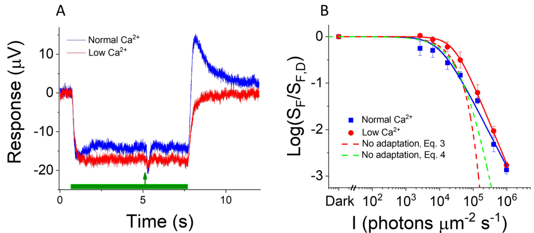
Figure 5. Ca 2+ -dependent and Ca 2+ -independent light adaptation mechanisms contribute to the light adaptation capacity of cones lacking both GCAPs and recoverin. (A) A response to a step of light ( I = 17,100 photons \mu\text{m}^{-2} \text{s}^{-1} ) superimposed with a test flash (arrow) recorded from GCAPs/recoverin-deficient cones in normal (blue) and low (red) Ca 2+ (same retina). The test flash strength was 1,600 and 570 photons \mu\text{m}^{-2} in normal and low Ca 2+ , respectively. (B) Sensitivity of cones ( S_F ) normalized to the sensitivity in darkness ( S_{F,D} ) plotted as function of background light intensity ( I ) for GCAPs/recoverin-deficient cones in normal (blue squares) and low (red squares) Ca 2+ . Smooth lines plot Eq. (2) with I_0 = 10,200 photons \mu\text{m}^{-2} \text{s}^{-1} and n = 1.4 in normal Ca 2+ (blue) and with I_0 = 27,000 photons \mu\text{m}^{-2} \text{s}^{-1} and n = 1.7 in low Ca 2+ (red). The dashed red and green traces plot Eqs (3) and (4), respectively, with parameter values calculated from dark-adapted responses of these cones in low Ca 2+ . Sensitivity data (mean \pm SEM) in (B) is from 3 GCAPs -/- Rv -/- Gnat1 -/- mice for which we used identical background light intensities. The theoretical traces plot the mean values for the same 3 GCAPs -/- Rv -/- Gnat1 -/- mice. For comprehensive statistical analysis, see Table 1 and text.
