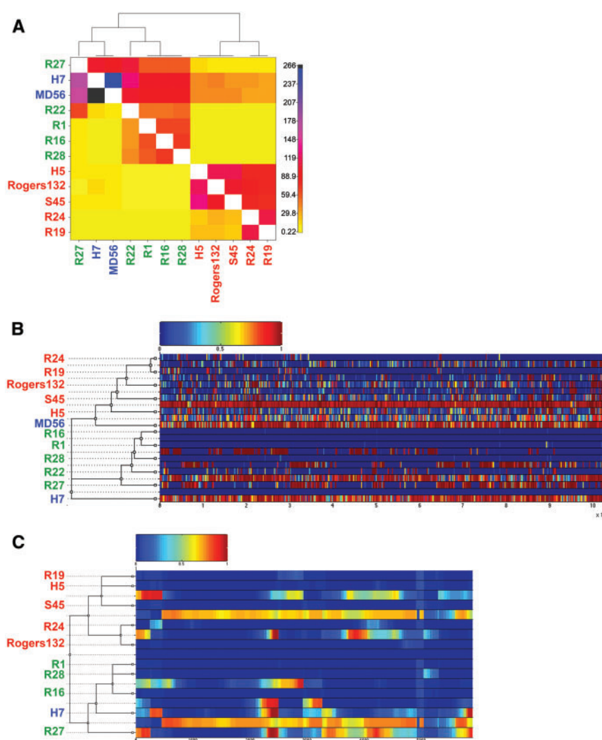
FIG. 2. —Frequent homologous recombination among Chlamydia suis (Cs) strains. (A) Abundant events of genetic exchange within the two Cs clades. ChromoPainter co-ancestry matrix with population structure was assignment based on fineSTRUCTURE analysis. The color of each cell of the matrix indicates the expected number of events (see vertical color bar on right) in which genetic material was copied from a donor genome (x axis) to a recipient genome (y axis). Clade 1 is shown in red, Clade 2 in green, and strains H7, and MD56 in blue; (B) Results of the ClonalFrame analysis on the chromosomes of 12 Cs genomes. Inferred clonal genealogy is shown on the left. Each branch of the tree corresponds to a row of the heat map, which is horizontally aligned according to the core MAUVE whole-genome alignment. Each row shows the posterior probability of recombination estimated by ClonalFrame on the corresponding branch (y axis) and along positions of the alignment (x axis); and (C) Results of the ClonalFrame analysis of 10 Cs plasmids. Strains R22 and MD56 were not included in this analysis because R22 does not possess a plasmid and plasmid contigs could not be distinguished from other contigs for MD56. Clade 1, Clade 2, and strains H7 and MD56 are shown in red, green and blue, respectively.
