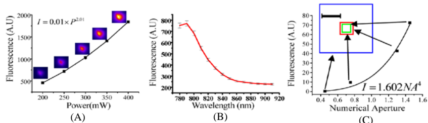
Fig. 2. Optical characteristics of wide-field two-photon excited fluorescence: (A) power dependence of the fluorescence of gallium corroles (50 \mu M) (B) fluorescence intensity versus wavelength of the mouse intestine stained with Alexa 568 phalloidin [power density: 64 \mu W/ \mu m 2 , ex: 780-910 nm (step: 10 nm), em: 620 \pm 60 nm, and a 40x air objective]. (C) fluorescence intensity versus numerical aperture of the objective lens [ex: 780 nm, power density: 64 \mu W/ \mu m 2 , 10x (NA: 0.45, FOV: 256 \mu m x 244 \mu m), 40x (NA: 0.75, FOV: 64 \mu m x 61 \mu m), 40x (NA: 1.30, FOV: 64 \mu m x 61 \mu m), and 60x (NA: 1.45, FOV: 43 \mu m x 41 \mu m)]. The rectangles represent the size of FOV.
