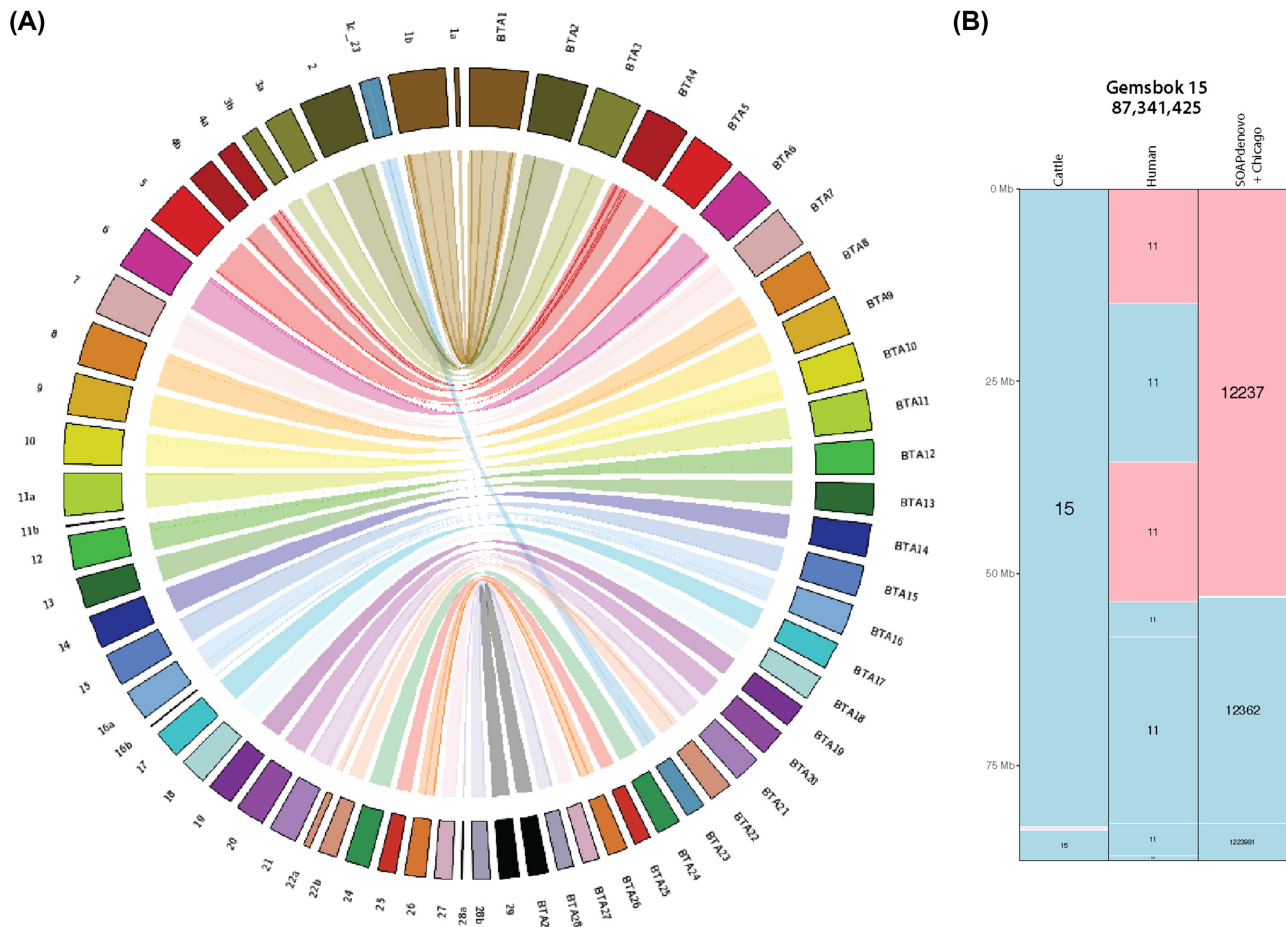
Figure 4: Syntenic relationships between gemsbok and cattle genomes. (A) Circos plot showing syntenic relationships between cattle autosomes (labeled as BTA) and gemsbok chromosomal fragments. Chromosomes are colored based on cattle homologies. Ribbons inside the plot show syntenic relationships, while lines inside each ribbon indicate inversions. (B) Gemsbok chromosome 15 showing homologous synteny blocks (HSBs) between gemsbok, cattle, and human. SOAPdenovo + Chicago scaffolds are also displayed. The other gemsbok chromosomes can be found in Supplementary Fig. S1.
