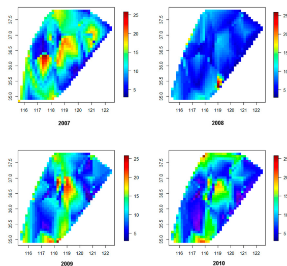
Figure 3. Temporal distributions of WQIs in the study area.
