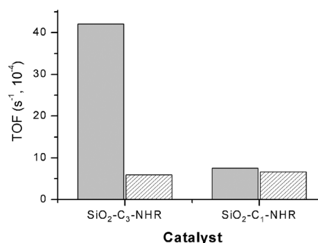
Figure 7. Effect of linker length on the catalytic activity of silica-supported secondary amine catalysts (solid bars) and comparison with their silylated analogs (striped bars). P_{\text{total}} = 1\text{ atm} ; P_{n\text{-butanal}} = 0.2\text{ kPa} , balance He; total gas flow rate = 150\text{ cm}^3\text{ min}^{-1} ; T = 343\text{ K} ; \text{SiO}_2 -823K; amine loading = 0.4\text{ -amine nm}^{-2} .
