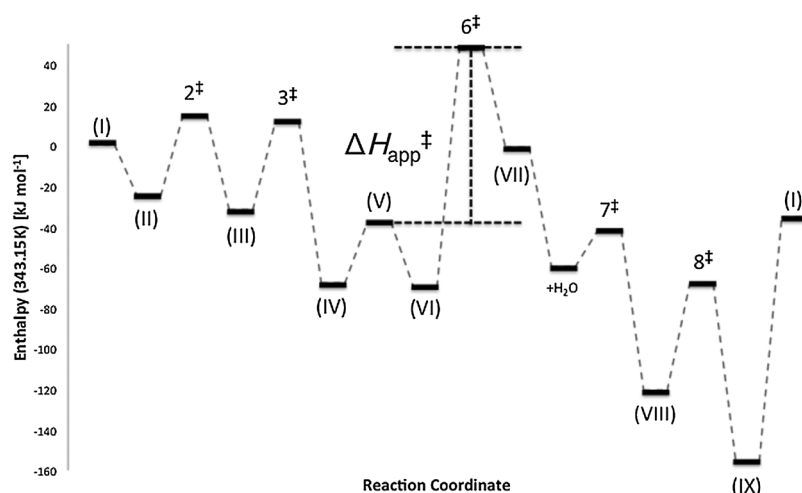
Figure 9. Enthalpy (343.15 K) diagram for aldol condensation of n -butanal over a SiO 2 -C 3 -NHR catalyst calculated at the ωB97X-D/6-311++G(3df,3pd) level of theory (kJ mol -1 ). The elementary steps are labeled according to the reaction mechanism in Scheme 1. The calculated apparent activation energy ( \Delta H_{app}^\ddagger ) is 85 kJ mol -1 .
