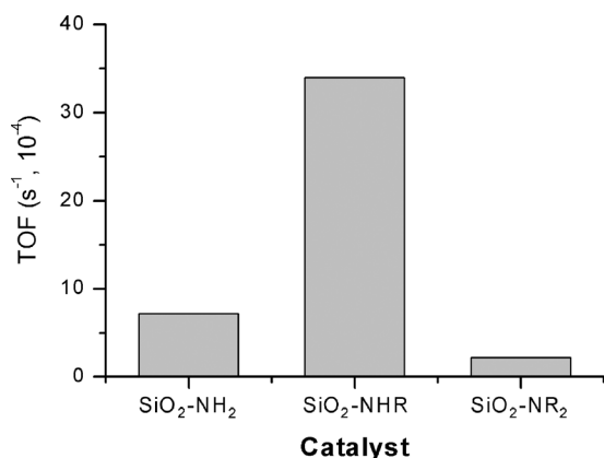
Figure 1. The effect of amine composition on the rate of 2-ethylhexenal synthesis over silica-supported amine catalysts P_{\text{total}} = 1 atm; P_{n\text{-butanal}} = 0.2 kPa, balance He; total gas flow rate = 150 \text{ cm}^3 \text{ min}^{-1} ; T = 343 K; amine loading = 0.4 \text{ -amine nm}^{-2} , TOF = turnover frequency.
