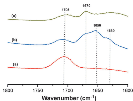
Figure 2. In situ FTIR spectra of n -butanal adsorbed at 343 K on silica-supported amine catalysts: (a) SiO 2 -NR 2 ; (b) SiO 2 -NHR, and (c) SiO 2 -NH 2 .
