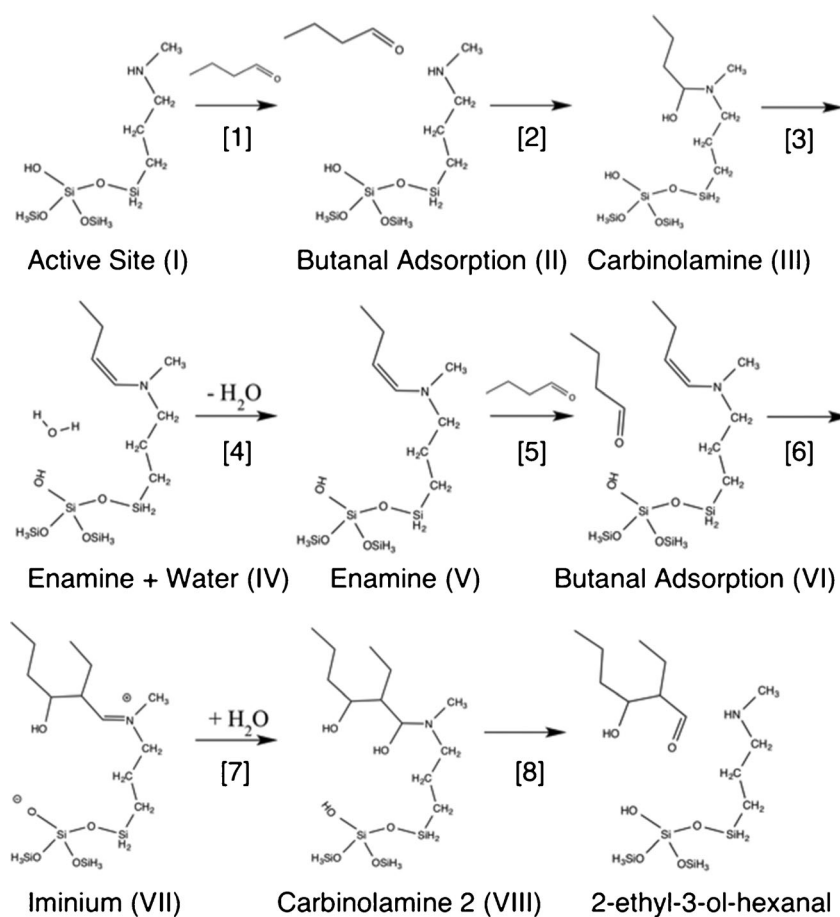
Scheme 1. Proposed mechanism for aldol self-condensation of n -butanal over silica-supported secondary amine catalysts.
