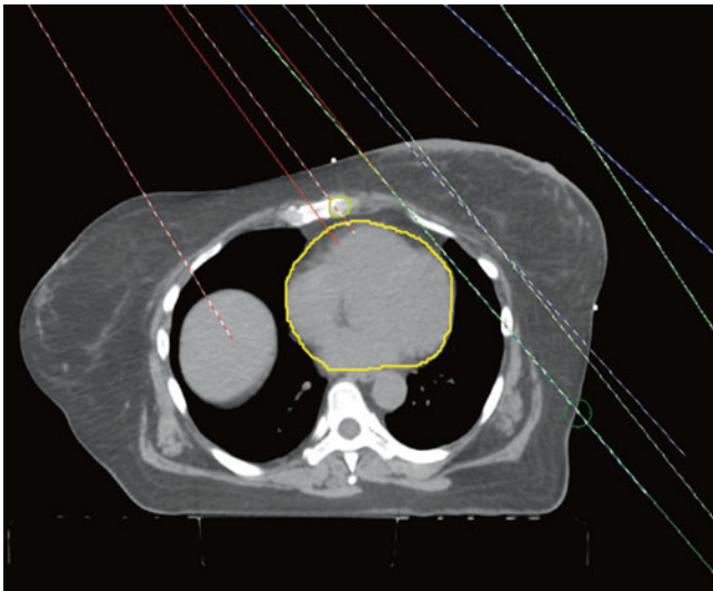
Fig. 7 Axial view of three beams: a medial en face electron beam (red) matched to two lateral opposing tangent fields (blue and green)
