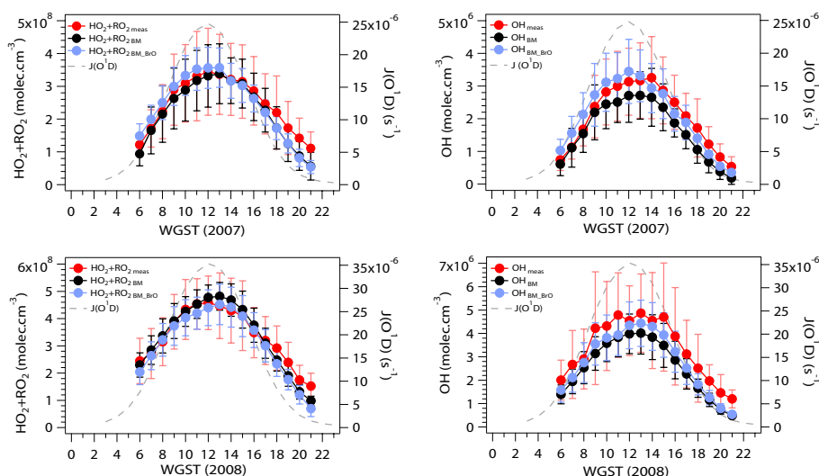
Fig. 7. The average diurnal profiles of hourly OH and HO 2 + RO 2 observations (red dots and line) and predictions from the BM (black dots and line) and BM.BrOCIMS (blue dots and line), and diurnal profile of J(O 1 D) (gray dash line) in spring 2007 and summer 2008. The error bars (red) of the observations are the overall uncertainties including the measurement uncertainties and ambient fluctuations. The error bars (gray and blue) of the predictions are the propagated uncertainties from the model input uncertainties and variations.
