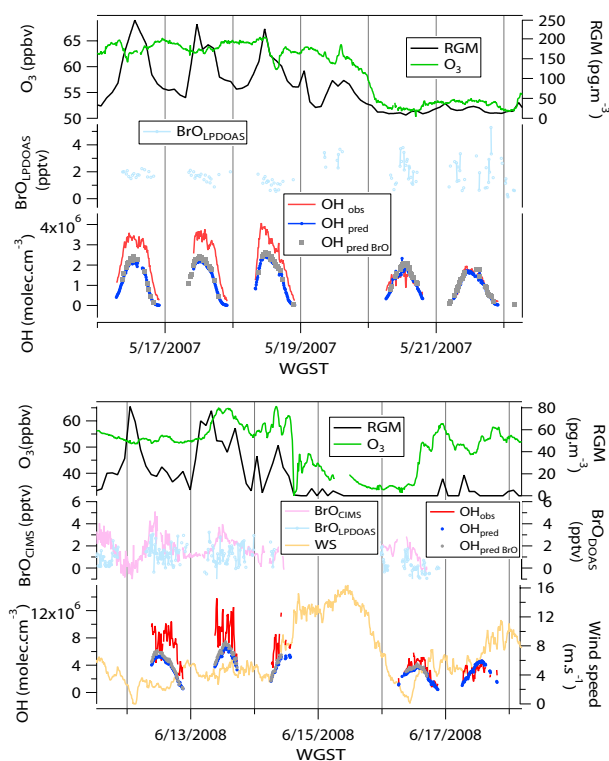
Fig. 9. (a): Observations of RGM, O 3 , BrO by DOAS and OH, and predictions of OH from the BM and BM.BrO when enhanced RGM were observed in 2007 (16 May–21 May 2007); (b): The observations of RGM, O 3 , OH, wind speeds, BrO by CIMS and DOAS, and the predictions of OH from the BM and BM.BrO when enhanced RGM were observed in 2008 (11 June–17 June 2008).
