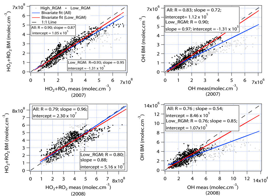
Fig. 8. The correlation plots of observed and predicted OH and HO 2 + RO 2 from the BM at low RGM conditions (black dots) and at high RGM conditions (gray dots) in 2007 and 2008. “All” represents the total data including low RGM and high RGM conditions. Equally weighted bivariate regressions are applied to all the data (blue line) and the data at low RGM conditions (red line), respectively. The relevant correlation coefficients, slopes, and intercepts are provided in the figure.
