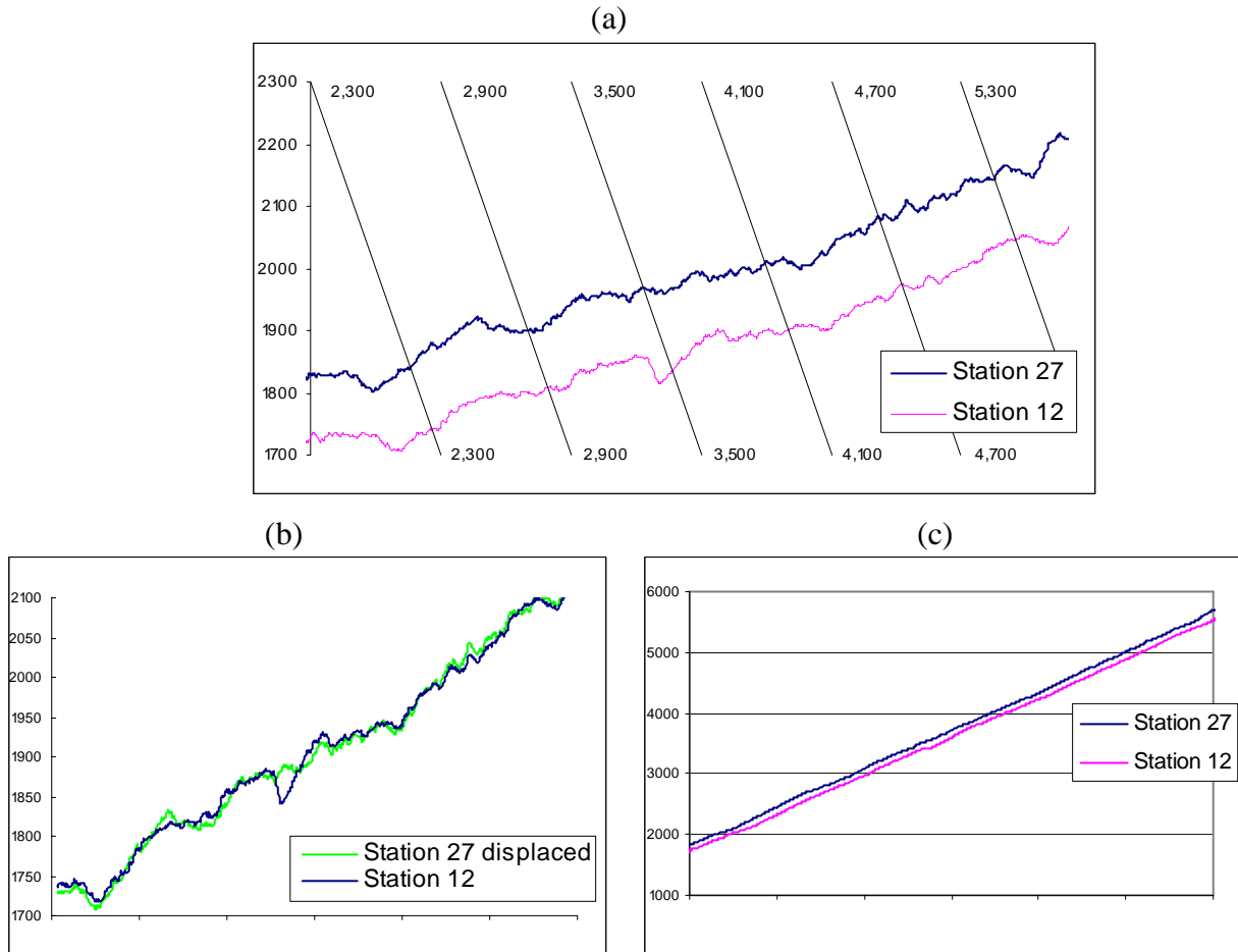
Figure 4. Traffic conditions at stations 12 and 27 between 14:15 and 14:45 hrs. (a) Oblique N-plot (background flow = 6930 vph); (b) shifted N-plot with N_{27} displaced along the oblique coordinates toward N_{12} (shift corresponds to a speed of 100 km/hr); (c) Ordinary N-plot.
