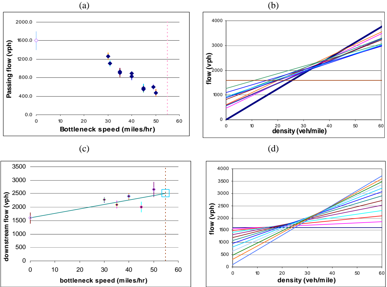
Figure 6: (a) Average passing rate and standard deviation estimated from measurements for different bottleneck speeds. (b) capacity lines on the density-flow plane obtained from the experimental data (c) Downstream (capacity) flow v/s bottleneck speed (d) Family of capacity lines generated by a linear relation between bottleneck speed and downstream flow
