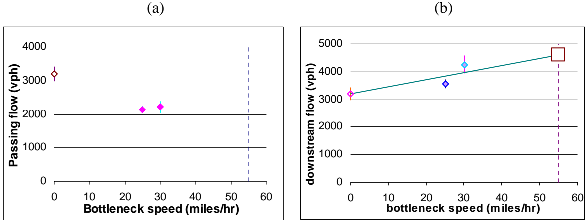
Figure 7: (a) Average passing rate and standard deviation estimated from measurements for different bottleneck speeds. (b) Downstream (capacity) flow v/s bottleneck speed.
