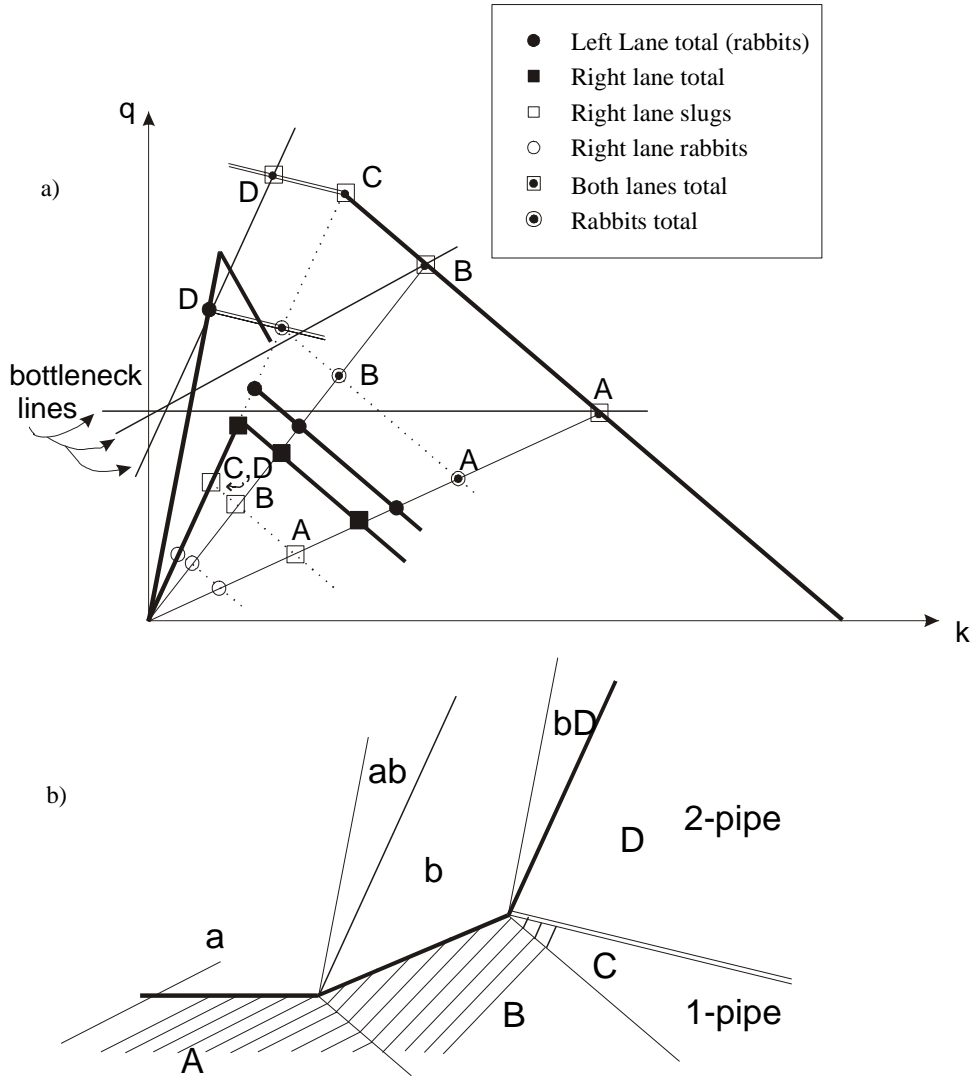
Figure A1: Solution of a problem where a bottleneck accelerates from a standstill until it reaches the desired speed of the slowest vehicles. a) Flow-density diagram, b) Time-space diagram.
