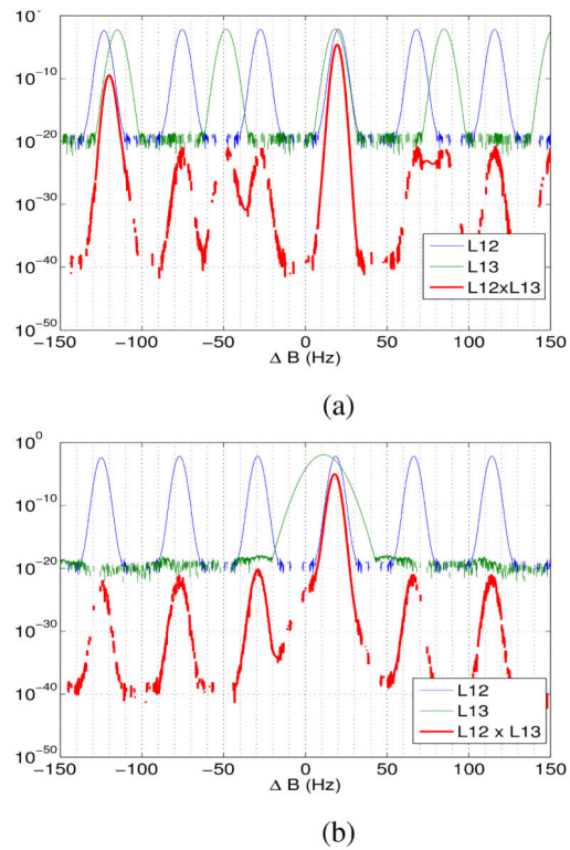
Figure 3. Example system likelihood functions obtained from individual dual-echo likelihoods. Note that the system likelihoods (red) are not subject to the same noise-phase wrapping trade offs as the dual-echo likelihoods (green and blue). That is, system likelihoods do not always possess multiple maxima whenever the function is multimodal.
