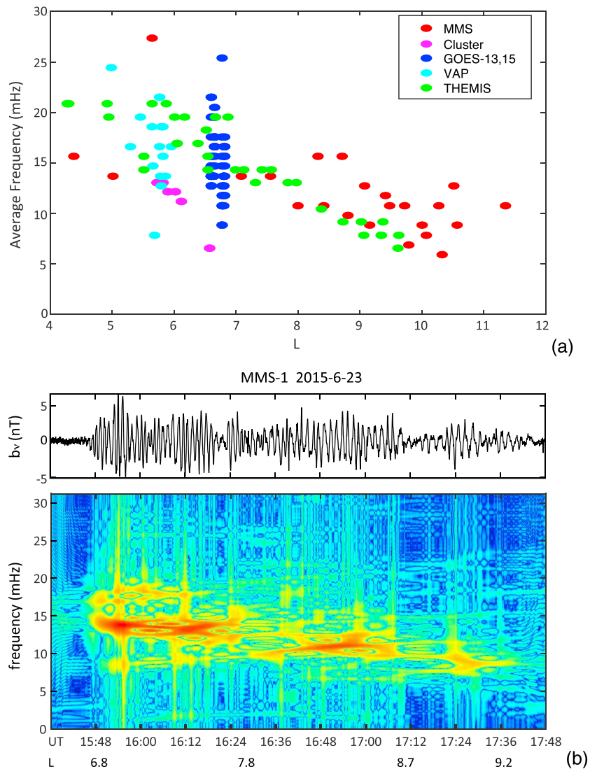
Figure 5. (a) average wave frequency as a function of L . (b) poloidal component of (top) the magnetic field and (bottom) the instantaneous wave frequencies estimated from Wigner-Ville distribution for the outbound pass of MMS-1 on 23 June 2015, covering the region with L from \sim 6.8 to \sim 9.2 in postdusk local times.
