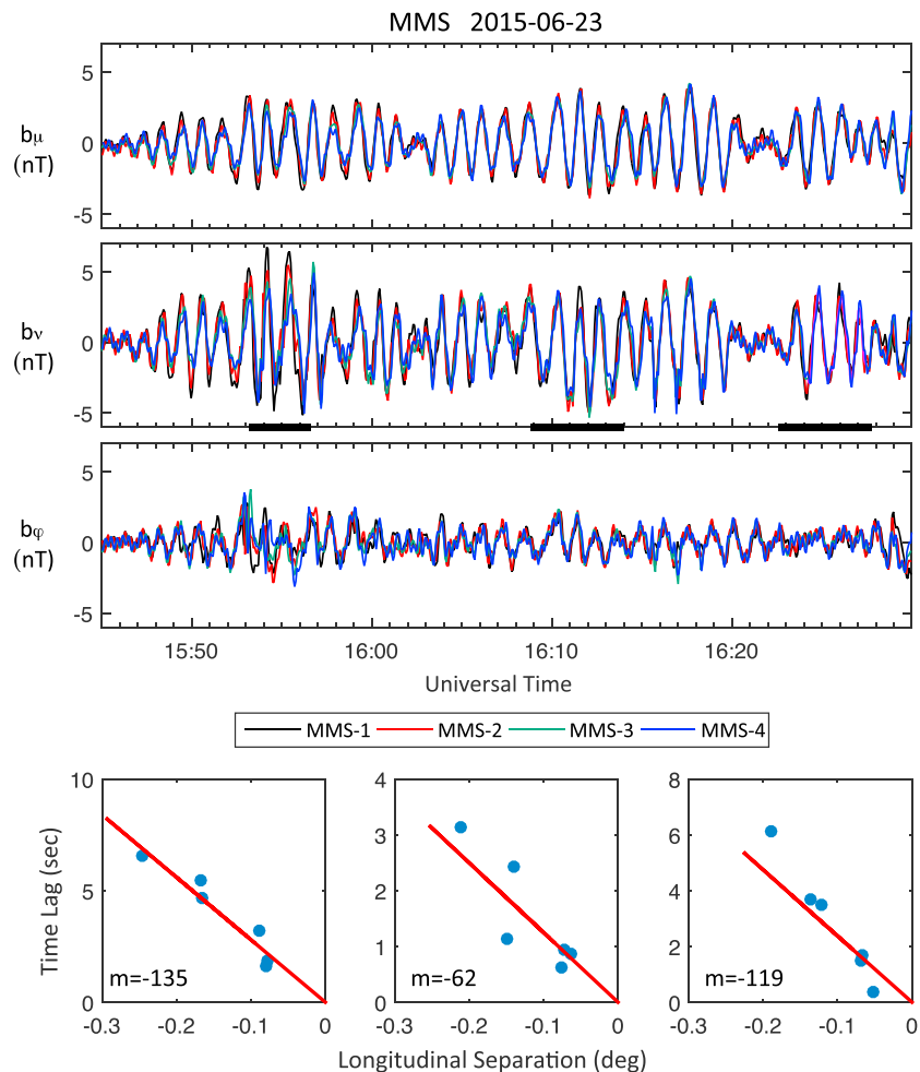
Figure 3. (first to third rows) MMS wave magnetic field in field-aligned ( \mu ), poloidal ( \nu ), and toroidal ( \phi ) directions. The three horizontal bars indicate the time intervals selected for estimating the azimuthal wavenumbers. (fourth row) The observed time lags in b_\nu versus longitudinal separations between MMS satellites.
