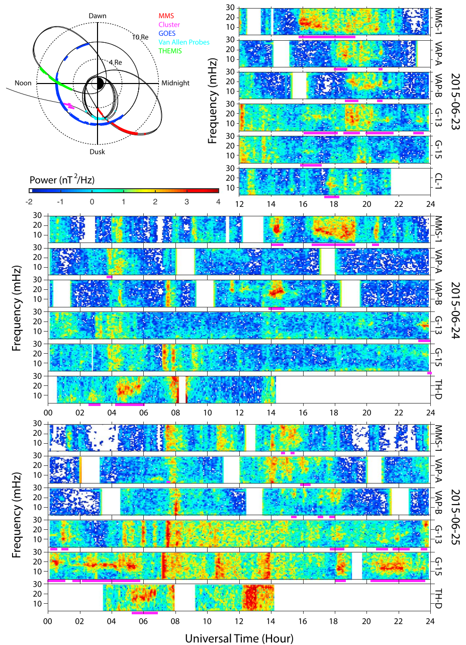
Figure 2. Spectrograms of poloidal component of the magnetic field ( b_1 ) observed by MMS, Val Allen Probes, GOES 13/15, Cluster, and THEMIS from 1200 UT, 23 June to the end of 25 June. Horizontal bars indicate the poloidal wave intervals. In the top left panel, the black traces are the satellite orbits, and color-coded segments are the locations of the wave intervals.
