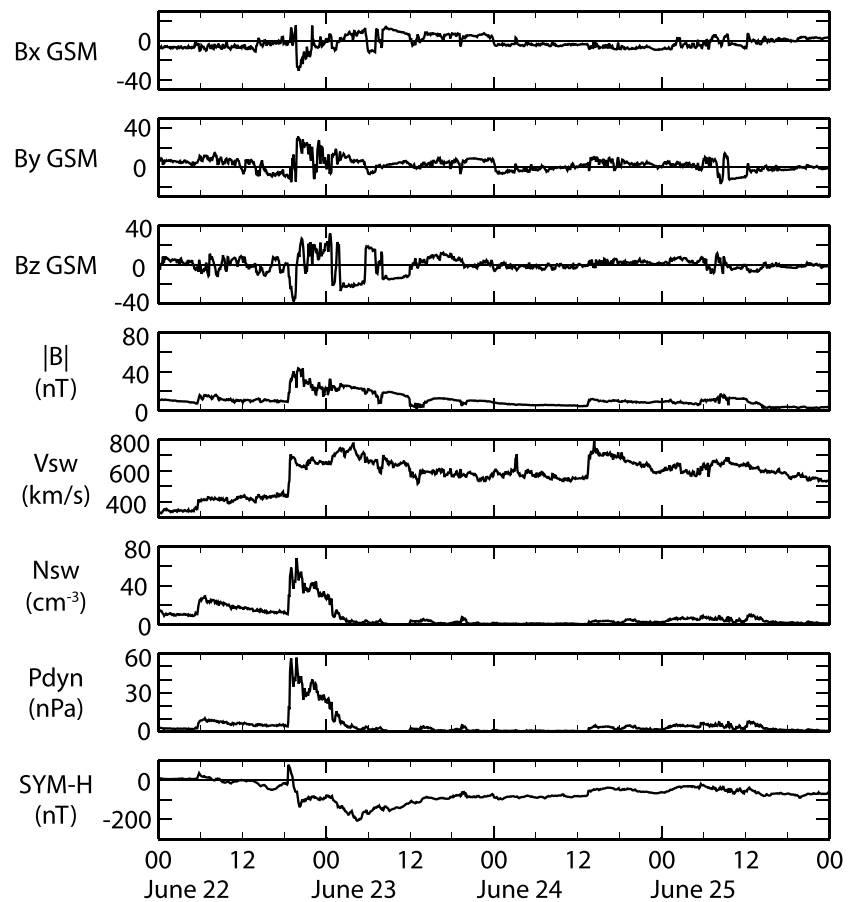
Figure 1. The IMF and solar wind data from ACE as well as the SYM-H index for the 22 June 2015 storm.
