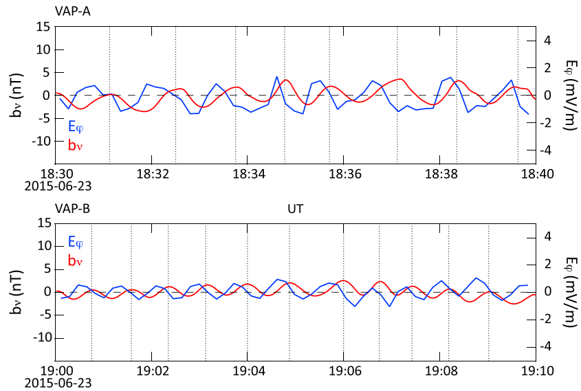
Figure 4. Poloidal component of the magnetic field (red) and azimuthal component of the electric field (blue) for two wave intervals observed by Van Allen Probes A and B, respectively. Vertical dotted lines are placed at peaks of b_v for guides only.
