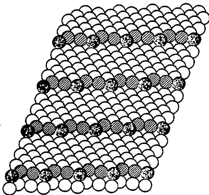
Fig. 6. Related to the stepped surface illustrated in Fig. 4 is the stepped-kinked surface shown above. This has the notation 7(111)\times(310) . The clear circles represent the so-called terrace or (111) type planes. Every seventh row a one atom step is encountered but this row is uneven with every third (dark shaded circles) atom a kink atom. Kink atoms have a coordination number of six.
