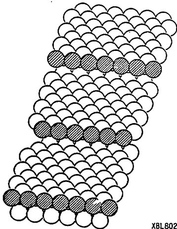
Fig. 5. This is a stepped surface for a face-centered cubic metal. One notation used for this surface is 9(111) \times (111) : the surface is generated basically from the (111) plane but every ninth row is a step and the steps are one atom high. The step atoms shown as black circles have a coordination number of seven. All atoms of this surface represented here by unshaded circles are in (111) environments.
