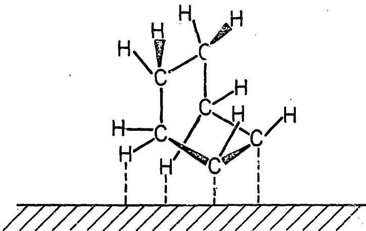
Fig. 9. The presumed initial chemisorption state of cyclohexene on a flat metal surface is shown here. Initial bonding should largely involve the \pi and \pi^* orbitals of the olefinic function so that the olefin C-C bond vector should be parallel, or nearly so, to the surface plane. Irrespective of the conformation of the C_6 ring, some aliphatic C-H hydrogen atoms should be near to the surface plane and these C-H bonds should be susceptible to facile cleavage.
