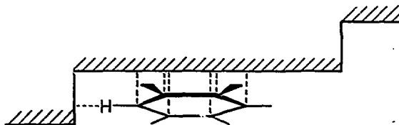
Fig. 8. This schematic representation for \pi bound benzene on a stepped or stepped-kinked surface illustrates the potential close approach of C-H hydrogen atoms to surface step atoms.
