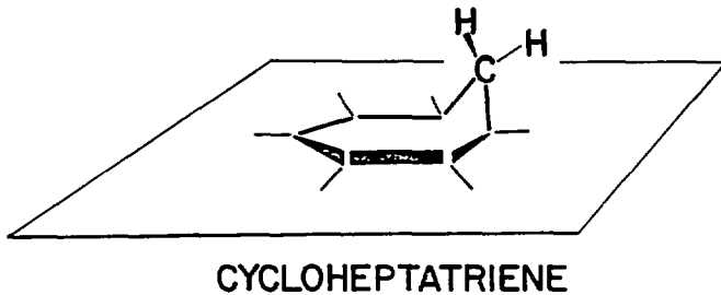
Fig. 10. Illustrated above for cycloheptatriene chemisorbed on an atomically flat surface plane is one possible stereochemistry in which none of the C-H hydrogen atoms can closely approach the surface metal atoms—a feature that would seem to be required for Ni(100)-C 7 H 8 because a significant fraction of cycloheptatriene chemisorbed on Ni(100) can be thermally desorbed.
