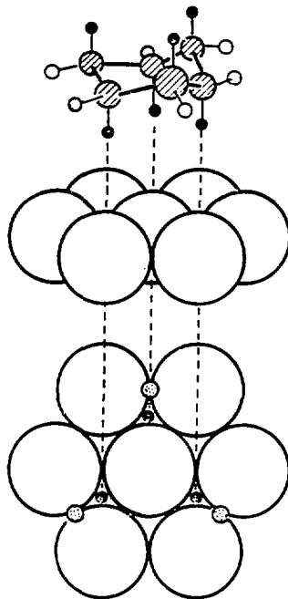
Fig. 11. A representation of the interaction of cyclohexane (chair form) with Ru(0001) as suggested by Madey and Yates (Ref. 18) in their classic study of hydrocarbon chemisorption on this basal plane of ruthenium. Three Ru-H-C three-center bonds are formed with three of the axial hydrogen atoms on one side of the chair form of cyclohexane. Weaker three-center Ru-H-C bonds may also be present with equatorial C-H hydrogen atoms.
