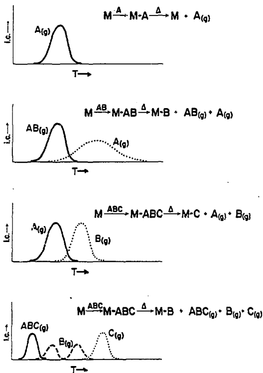
Fig. 1. Illustrative but hypothetical desorption spectra for molecules chemisorbed on a metal surface. Plotted is the ion current for the parent mass ion derived from the gaseous species desorbed from the surface as a function of temperature (line shapes are a function of crystal heating rates among other factors). The top spectrum is the idealized fully reversible adsorption, a situation rarely encountered except for hydrogen, nitrogen, carbon monoxide (electronegative metals), and some saturated hydrocarbons. Following is the desorption spectrum for a system in which the adsorption is only partially reversible; a common example found in surface chemistry is that for hydrocarbons where A represents carbon and A(g) would represent H_2(g) . The third spectrum comprises fully irreversible chemisorption; an example is Ni(111)-C_6H_5CH_3 which primarily yields H_2 at low temperatures and N_2 at high temperatures to leave a Ni(111)-C surface. The last spectrum illustrates competing reversible thermal desorption and thermal decomposition. Note that in the last spectrum B(g) shows two thermal desorption maxima. This type of spectrum with two B(g) desorption maxima is sometimes observed for hydrocarbons on metal surfaces where B(g) is H_2(g) ; a specific example discussed in the text is the decomposition of toluene on atomically flat metal surfaces.
