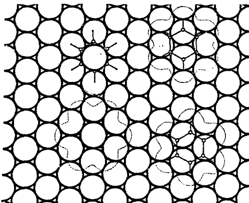
Fig. 7. An infinite array of registries for Ni(111)-C 6 H 6 are consistent with the low energy electron diffraction study of the ordered chemisorption state. Shown above are four idealized possibilities with the C 6 centroid centered over a single nickel atom, over two-fold sites and over three-fold sites. Each of the possible registries are consistent with the (2\sqrt{3} \times 2\sqrt{3})R30^\circ unit cell established by low energy electron diffraction studies and vibrational (high resolution electron energy loss) data. The benzene bond distances were derived from X-ray and neutron diffraction study of C 6 H 5 Cr(CO) 3 ; the dotted lines define the van der Waals outline of the benzene molecule. Because the distance between hydrogen atoms at para positions in the benzene molecule is virtually identical to twice the nickel atom diameter, the registry with the C 6 centroid atop a single nickel atom is precise (upper left and right). Overlaps with the \pi and \pi^* benzene orbitals and metal surface orbitals should be excellent. In one rotational form (upper right) the hydrogen atoms of the benzene lie directly over single nickel atoms so as to generate multicenter C-H-Ni bonds. The van der Waals extension of the benzene molecule (dotted line) is virtually identical with the space occupied by the central nickel atoms and the surrounding six nickel atoms. Another form generated from the above by a rotation of 30^\circ has the C-H hydrogen atoms lying nearly above the two-fold sites (upper left). Either of these may be the most stable registry for benzene on this surface.
