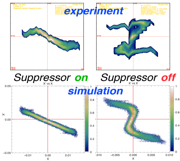
Fig. 3.2: Optical slit scanner plots of the ion beam phase space ( X, X' ). (a) Experiment with the electron suppressor on. (b) Experiment with the electron suppressor off. (c) Numerical simulation for the electron suppressor on. (d) Simulation for the electron suppressor off.
