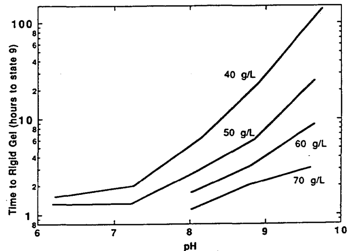
Fig. 3. Time to rigid gel (state 9) of CS-B with varying concentrations of added NaCl and varying pH.
