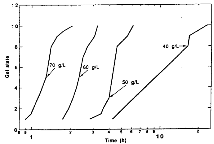
Fig. 2. Gel-time jar test of CS-B with varying concentrations of added NaCl, pH adjusted to 8.9 (the natural buffered pH of Hanford sand). The vertical axis is a visual assessment of gel state, modified from Sydansk (8).
