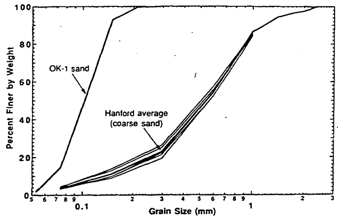
Fig. 1. Particle size analyses of sands used in this study.
