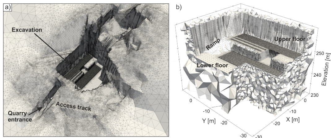
Figure 5. Discretization of the quarry domain. (a) View of the extended model showing the quarry surroundings, including the access track and the quarry entrance. The excavation has dimensions of 30 \times 40 m. (b) Subset showing the discretization of within the imaging area, showing the mesh refinement around the electrode locations and the modelling of the quarry interior.
