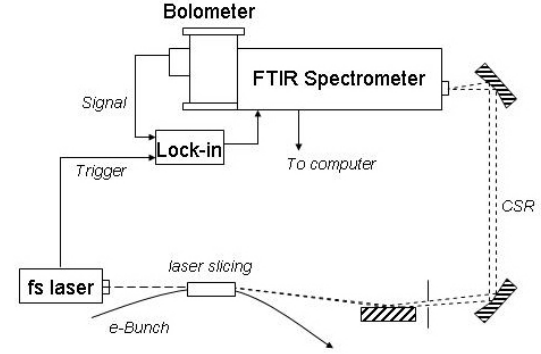
Figure 3: A schematic of the measurement apparatus.
