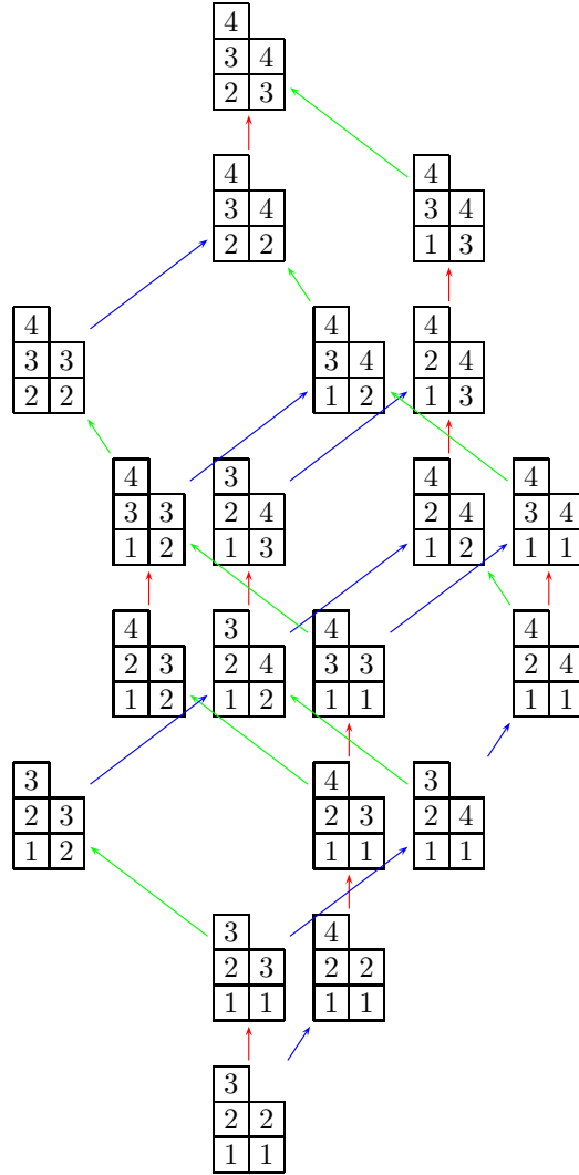
FIGURE 3. The crystal B(2, 2, 1) , with edges f_1 \leftarrow , f_2 \uparrow , f_3 \rightarrow .
