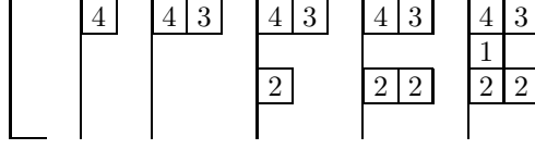
FIGURE 15. The weak recording tableau for the reduced factorization (4)(5)(23)(2) .
