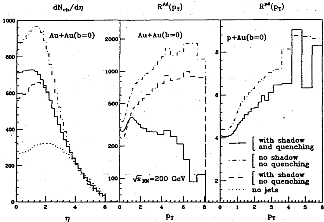
Figure 13. Results from HIJING calculations on the dependence of the inclusive charged hadron spectra in central Au + Au and p + Au collisions on minijet production (dash-dotted), gluon shadowing (dashed) and jet quenching (solid) assuming that the gluon shadowing is identical to that of quarks (see Ref. 56 for details). R^{AB}(p_T) is the ratio of the inclusive p_T spectrum of charged hadrons in A + B collisions to that of p + p.
