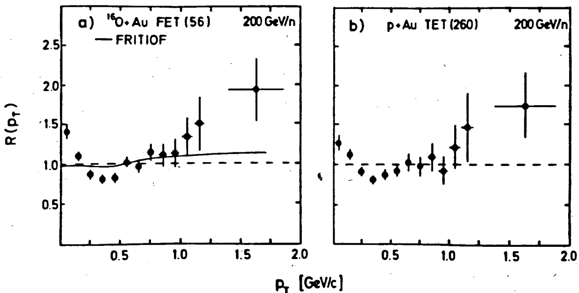
Figure 6. Ratios R(p_t) of the transverse momentum distributions of central a) ^{16}\text{O} + \text{Au} and b) p + Au collisions relative to minimum bias p + p collisions at 200 GeV/n. The dashed lines indicate R(p_t) = 1 . The trigger conditions were a) forward energy trigger FET(56) and b) transverse energy trigger TET(260) with trigger cross sections of 56 and 260 mb, respectively.
