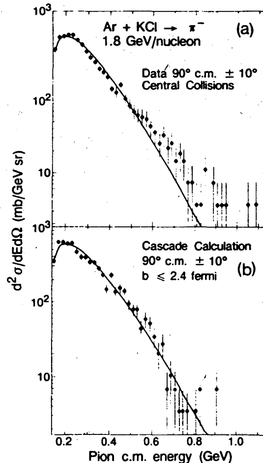
Figure 4. The energy spectrum of negative pions at 90^\circ in the c.m. system a) measured and b) calculated using the intranuclear cascade model. The solid curves are fits to the spectra using a Maxwell-Boltzmann distribution with pion temperatures a) T_\pi = 69 \text{ MeV} and b) T_\pi = 73 \text{ MeV} .
