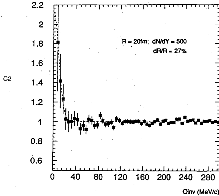
Figure 21. Correlation measurement for a single event simulated with R_{inv} = 20 fm and dN_{\pi^-}/d\eta = 500 in STAR at midrapidity.
