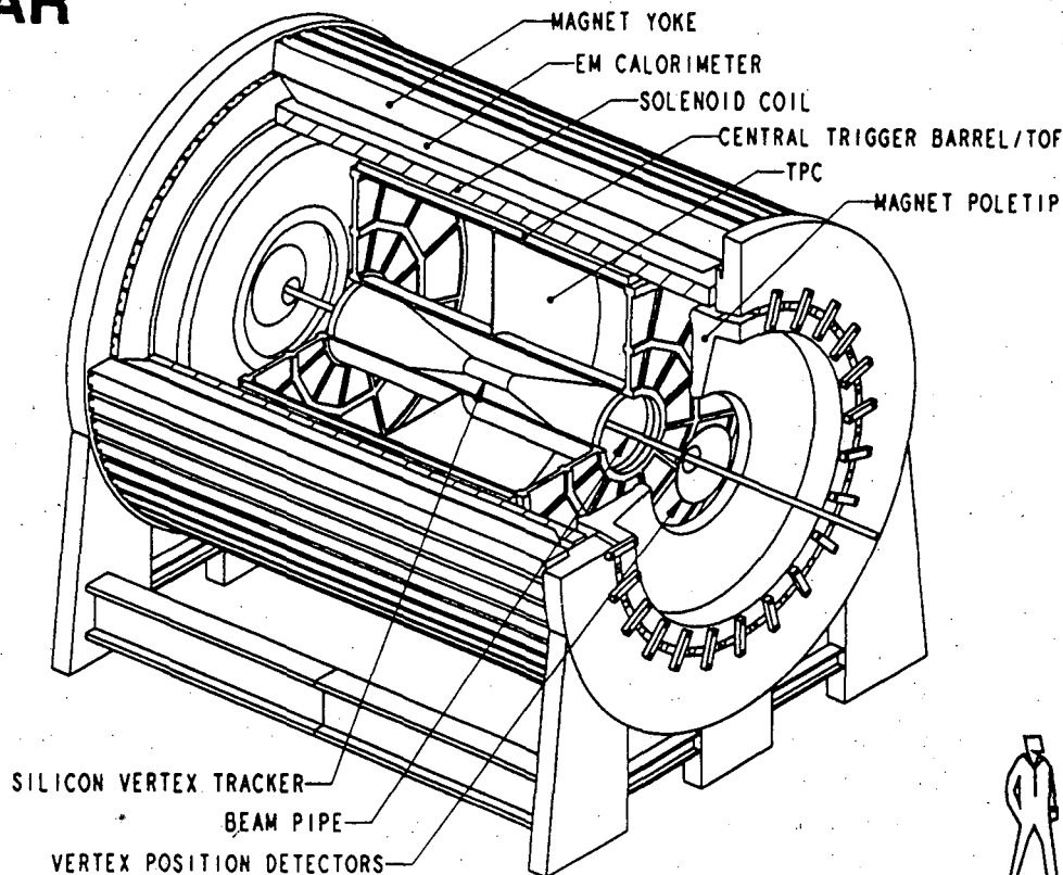
Figure 15. Conceptual layout of the experiment, with cylindrical symmetry around the beam axis. See text for description.
