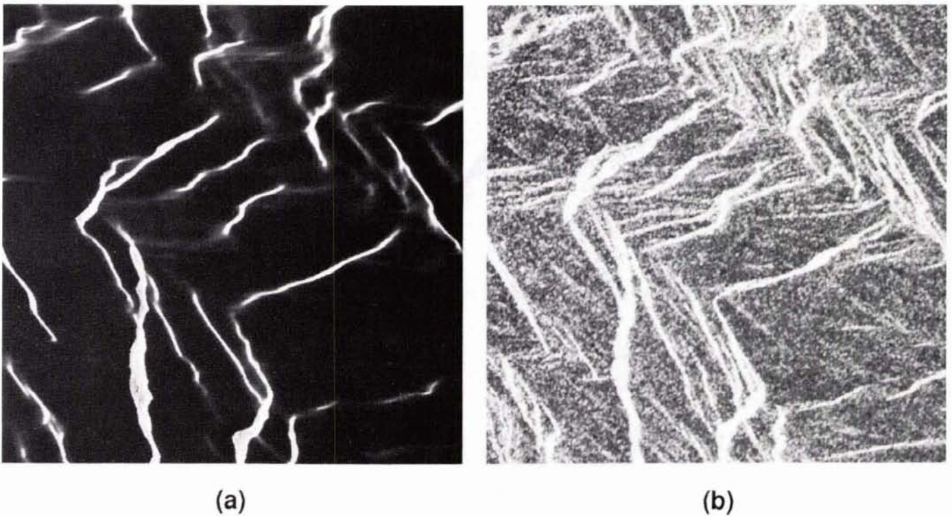
FIG. 4. Comparison of simulated versus actual Seasat SAR image; (a) simulated image; (b) actual image.
