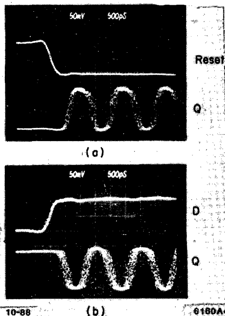
Fig. 4. Displays of asynchronous resetting of a NEC device 4 using both the RESET and D inputs for phase shifting.
