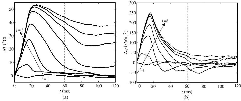
Figure 5. Dynamics of differences in (a) temperature and (b) heat flux between the centre of the spray surface and at other locations. Dashed line denotes end of cryogen spurt.
