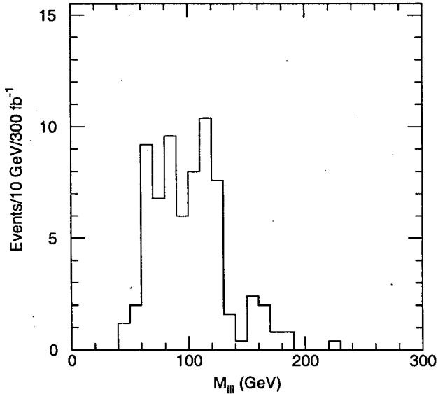
Figure 18: M_{\ell\ell} distribution after the cuts for the modified point with m_5 = 125 GeV.
