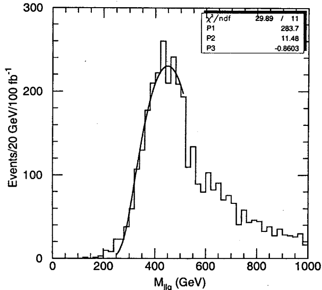
Figure 4: Distribution of the larger of the two llq masses after cuts described in the text, showing the lower edge.
