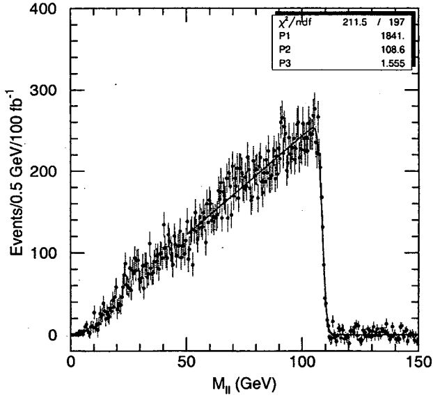
Figure 10: \ell^+\ell^- mass distribution showing the maximum likelihood MINUIT fit using PAW.
