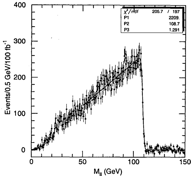
Figure 9: l^+l^- mass distribution showing the \chi^2 MINUIT fit using PAW.
