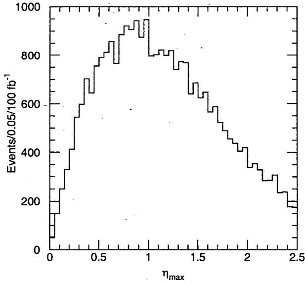
Figure 11: Maximum |\eta_\ell| for dilepton events.
