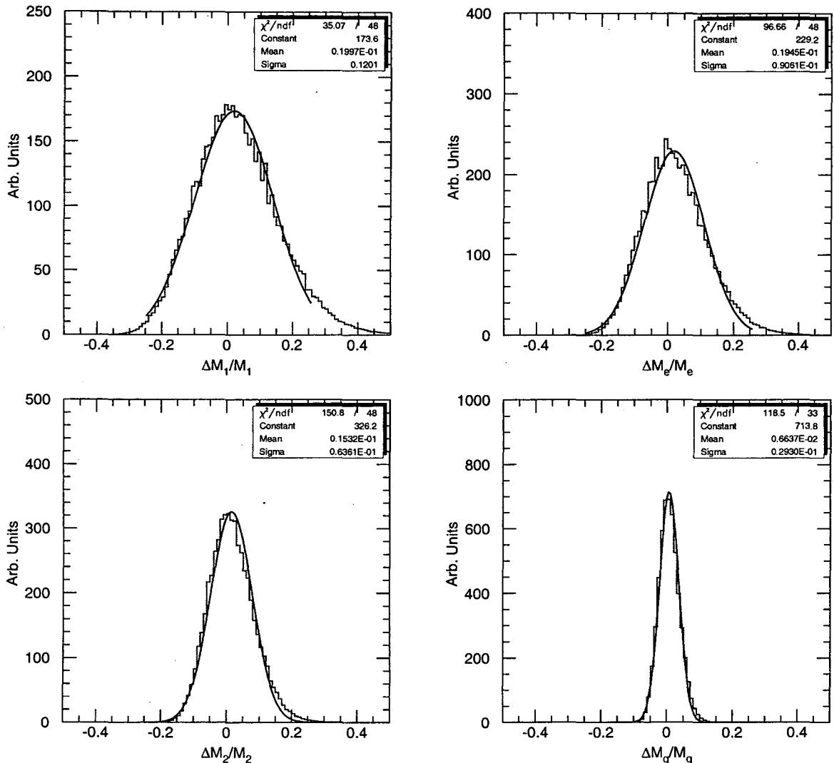
Figure 6: Distribution of the \tilde{\chi}_1^0 , \tilde{\ell}_R , \tilde{\chi}_2^0 , and \tilde{q}_L masses satisfying all constraints discussed in the text. The fitted widths are about \pm 12\% , \pm 9\% , \pm 6\% , and \pm 3\% respectively.
