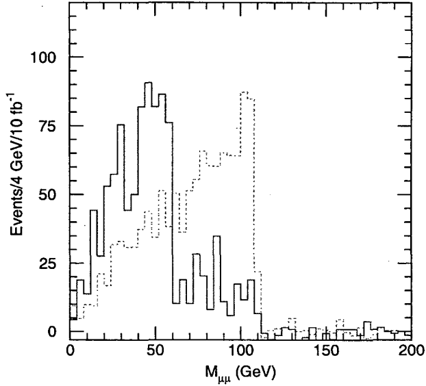
Figure 15: M_{\mu\mu} distribution after the cuts at the m_5 = m_{10} = 100 GeV point (dashed line) and modified point with m_5 = 50 GeV (solid line).
