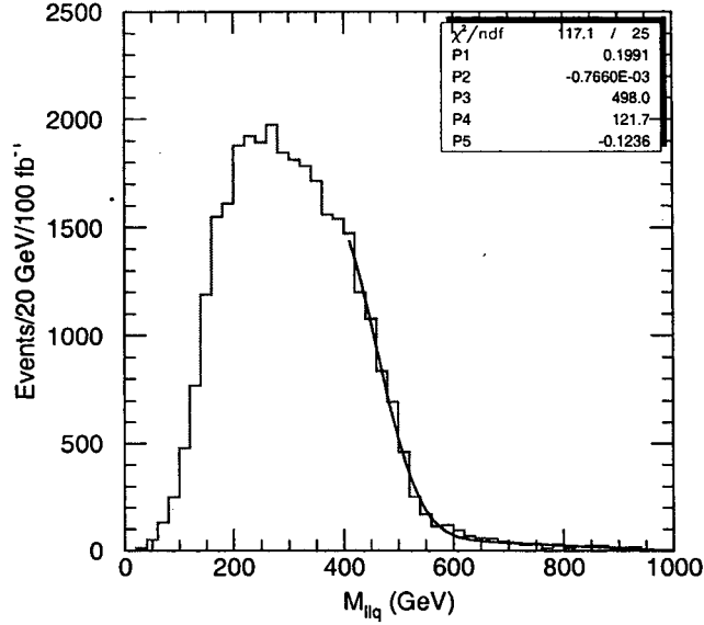
Figure 3: Distribution for the smaller of the two \ell^+ \ell^- q masses from Figure 1; a Gaussian-smearred fit plus a linear background described in the text is also shown.
