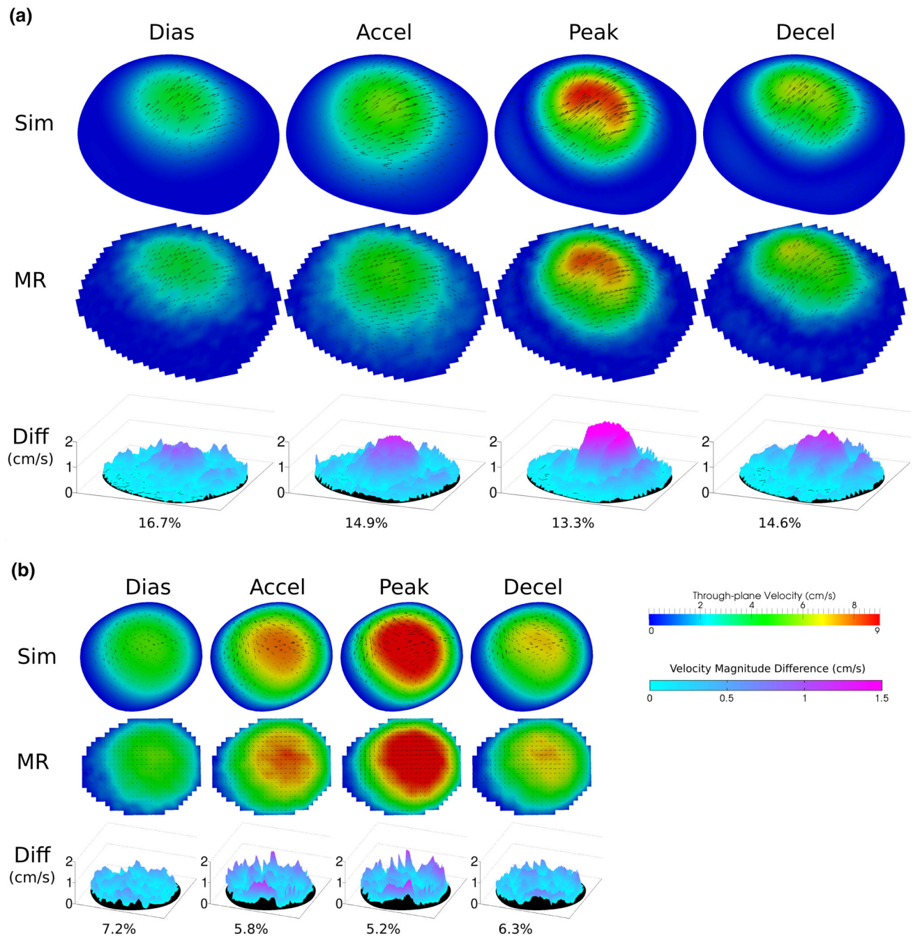
FIGURE 5. Resting condition flow velocity comparisons: between MR measurements and simulation results at diastole, acceleration, peak, and deceleration time point at slice locations (a) S1 and (b) S2. Color map and arrows correspond to through-plane and in-plane velocities, respectively. Velocity magnitude differences across the slices are shown as 3D surface plots. Percent difference in velocity magnitude averaged across the slice are also shown.
