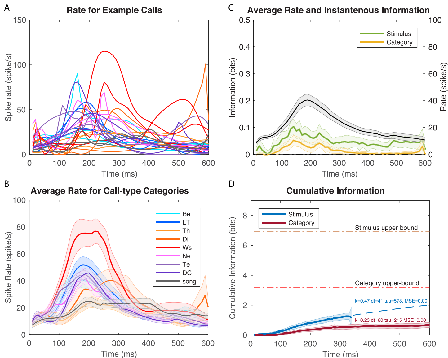
Fig 5. Time-varying firing rates and information values for example neuron 3. As in Fig 3 but for a neuron with intermediate firing rates and displaying selectivity for Wsst (Ws) or Aggressive Calls. Note also the longer latency relative to the neuron shown in 3 and 4. Spike rasters for this neuron are shown on S6 Fig. A. Time-varying firing rate obtained from KDE of ten repetitions of different example stimuli. B. Averaged time-varying firing rate obtained for each call-type category. C. Overall time-varying firing rate and instantaneous information for stimuli and call-type categories. D. Cumulative information for stimuli and call-type categories. See details in legend of Fig 3.
