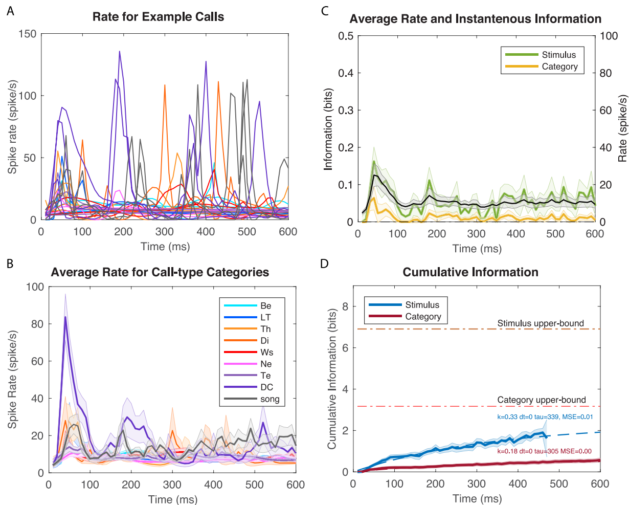
Fig 4. Time-varying firing rates and information values for example neuron 2. As in Fig 3 but for a neuron with lower firing rates and displaying selectivity for Distance Calls. Spike rasters for this neuron are shown on S5 Fig. A. Time-varying firing rate obtained from KDE of ten repetitions of different example stimuli. B. Averaged time-varying firing rate obtained for each call-type category. C. Overall time-varying firing rate and instantaneous information for stimuli and call-type categories. D. Cumulative information for stimuli and call-type categories. See details in legend of Fig 3.
