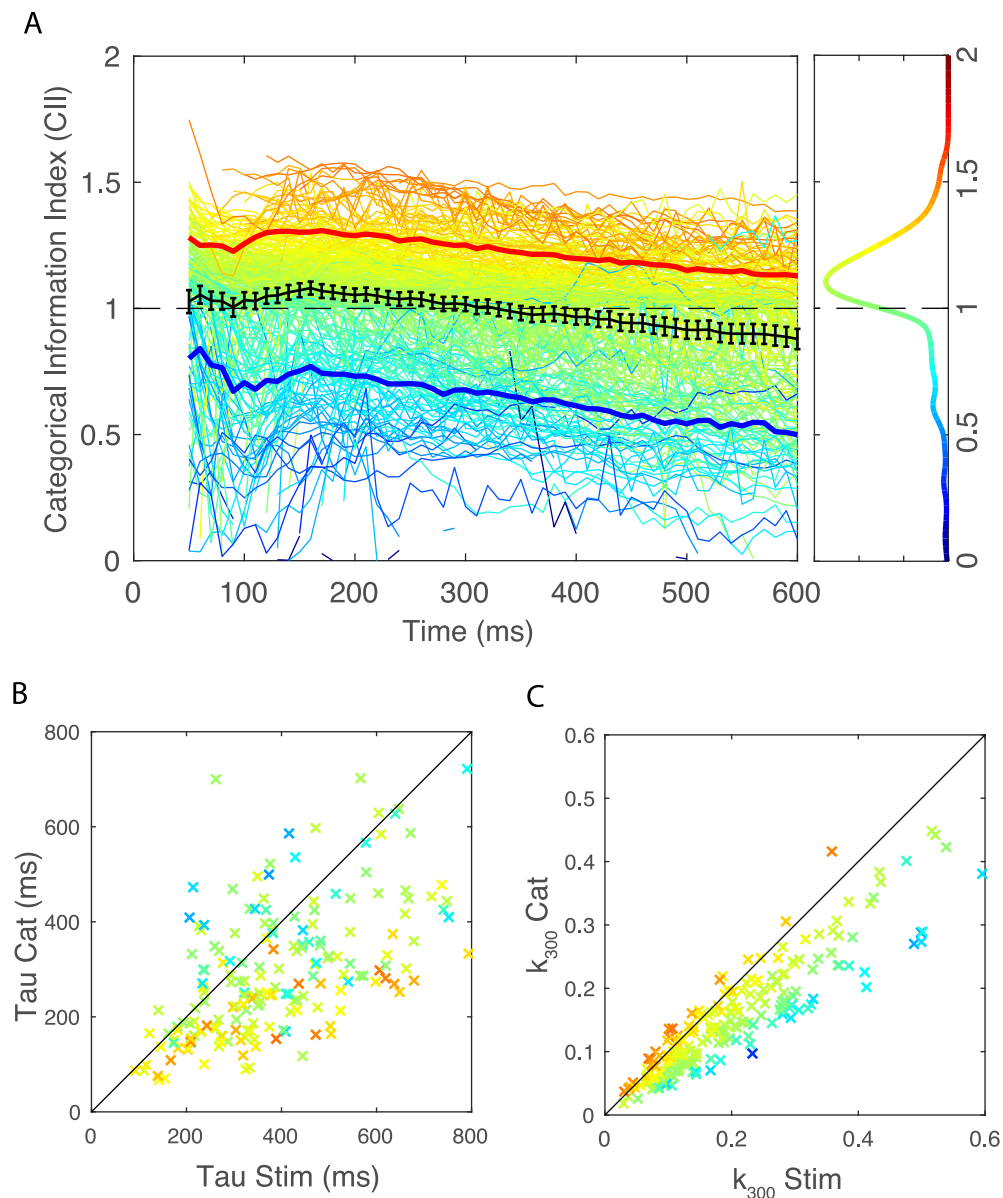
Fig 9. Categorical cumulative information index and its relationship to time constants tau and relative cumulative information estimate K_{300} . As explained in Fig 8 and in the text, the cumulative information (CI) for call-type categories can be analyzed in terms of a floor or minimum value, a shared value and a ceiling or maximum value. A Value of the Categorical Information Index (CII) as a function of time for all neurons in the population. Each line color corresponds to the time average CII of the neuron obtained between 50 and 300ms. The solid red line is the average obtained for the quartile of neurons with the highest CII and the blue solid line is average obtained for the quartile of neurons with the lowest CII. Error bars on the average CII (solid bold black line) are 2 SEM. The right vertical panel shows the distribution of CII at 150 ms. B Scatter plot of the time constant of the exponential fit for stimuli (Stim—x axis) versus call categories (Cat—y axis). C Scatter plot of k_{300} for stimuli (Stim—x axis) versus categories (Cat—y axis). Single data points in B and C are colored according to the time average CII of each neuron as in A.
