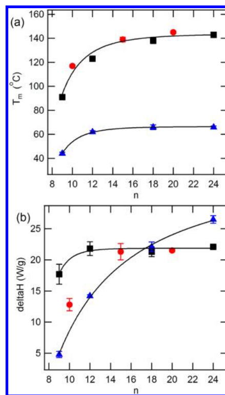
Figure 3. (a) Plots of T_m of pNdc and pNte in block copolypeptoids and homopolypeptoids by DSC versus n (chain length of pNdc block). (b) Plots of \Delta H of pNdc and pNte in block copolypeptoids and homopolypeptoids by DSC versus n (chain length of pNdc block). In both panels, red circles plot pNdc homopolypeptoids, blue triangles plot pNte blocks, and black squares plot pNdc blocks in block copolypeptoids.
