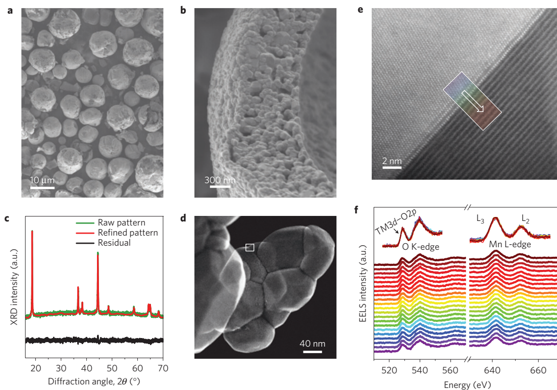
Figure 3 | Characterization of the NMC-442 materials synthesized by spray pyrolysis. a, b , SEM at different magnifications. c , XRD and Rietveld refinement. d-f , SEM-STEM-EELS, where a selected particle-particle interface marked in d was used for ADF-STEM imaging ( e ) and EELS O K-edge and Mn L-edge measurements ( f ). In the brighter particle (top left) in e , two domains that are \pi out of phase are projected in this image.
