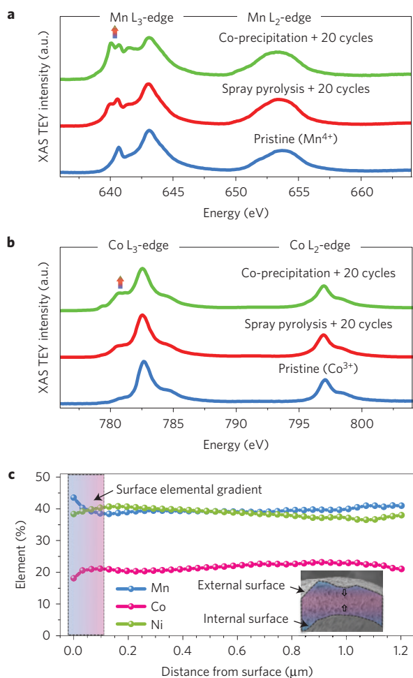
Figure 6 | Surface chemistry of NMC materials before and after electrochemical cycling. a,b , XAS spectra of Mn L-edge ( a ) and Co L-edge ( b ) of NMCs in the pristine state (blue) and after 20 charge-discharge cycles to 4.7 V versus Li/Li + (red and green), stopped in the discharged state. Transition metal L-edges are divided into L 3 and L 2 features located at lower and higher energy regions of the spectra, respectively. The small arrows point to the Mn and Co L 3,low edges, which increase in magnitude in cycled electrodes compared with pristine ones, indicating that the oxidation states of metals near the surfaces are lower in the former compared with the latter. The co-precipitation data are used with permission from ref. 11. c , Elemental distribution as a function of the distance from microsphere surface calculated using the TXM data, and the elemental distribution at the surface region is highlighted using the blue-magenta shadow. The distance from surface was calculated from both the internal and external surfaces of the hollow shell, as schematically shown in the inset.
