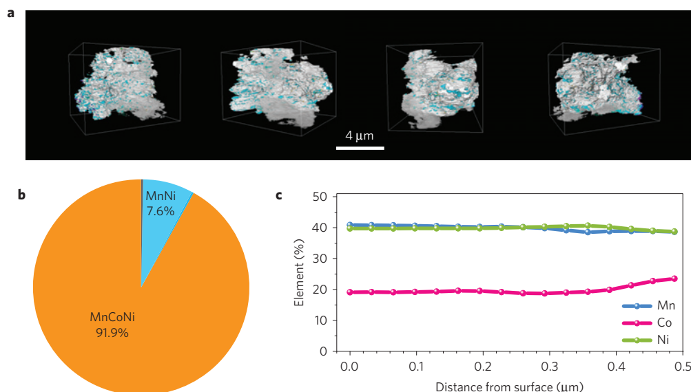
Figure 7 | 3D elemental association mapping and elemental distribution of co-precipitated NMC particles. a , Elemental association maps of a particle selected from the co-precipitated sample, where the cyan colour represents the regions where Co was not observed. b , The relative concentrations of 3D elemental associations calculated by using absorption correlation tomography; elemental associations other than MnCoNi and MnNi were all below 1% such that they are negligible in the pie chart. c , Elemental distribution as a function of the distance from the secondary particle surface calculated using the TXM data, in direct comparison with Fig. 6c.
