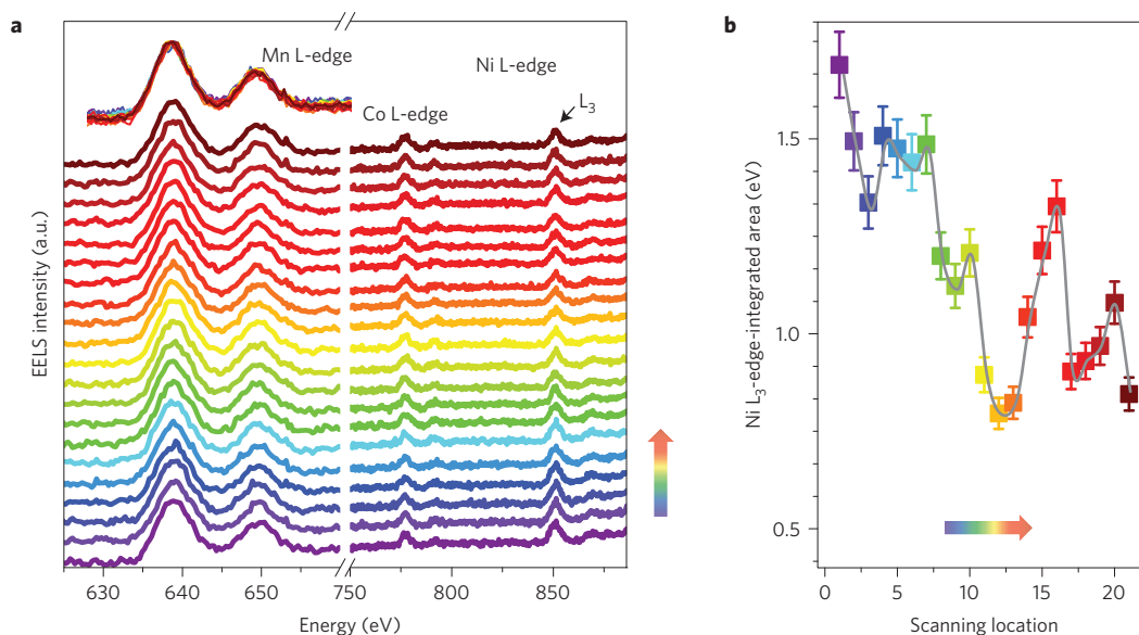
Figure 4 | Electronic and compositional characterization using EELS. a , Transition metal L-edge EELS spectra along the scanning pathway shown in Fig. 3e, where the spectra were normalized using the Mn L-edge. The normalized spectra were overlapped on the top of the stacked spectra, demonstrating the identical peak characteristics for all of the Mn L-edge spectra. b , The Ni L_3 -integrated areas calculated after the Mn L-edge normalization. The error bars are based on multiple peak area calculations and the line is to assist visualization. The coloured arrows in the figure represent the scanning direction corresponding to the one in Fig. 3e.
