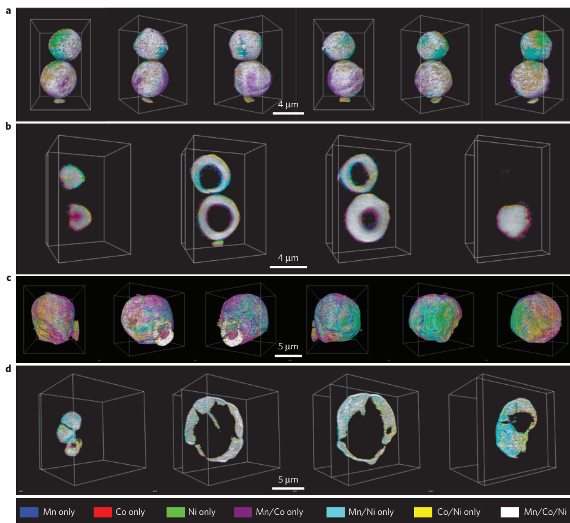
Figure 2 | 3D elemental association maps generated using transmission X-ray tomography. a–d. Elemental association maps of the as-made NMC precursor after spray pyrolysis ( a,b ) and the powder after annealing at 850 °C ( c,d ). a,c , 3D rendering of the elemental associations viewing the particles at different angles, where the visualization is enhanced in Supplementary Video 3 for the powder after annealing at 850 °C. b,d , 2D slices of the elemental associations cut through at different depths of the imaged particles. The colours representing the elemental associations are shown at the bottom.
