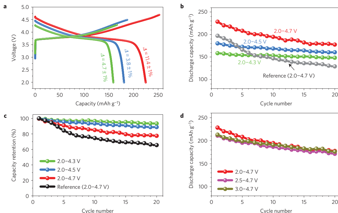
Figure 5 | Battery cycling performance of lithium half-cells containing the NMC-442 materials. a , First charge–discharge cycles between various voltage cutoff windows with percentage Coulombic inefficiencies indicated. Red, blue and green lines represent voltage limits of 2.0–4.7 V, 2.0–4.5 V and 2.0–4.3 V, respectively. These cells were cycled at approximately similar rates. b , Discharge capacities as a function of cycle numbers during the galvanostatic cycling, with reference data taken from ref. 21 on an NMC-442 material prepared by a glycine–nitrate combustion method and cycled between 2.0–4.7 V. c , Discharge capacity retention at various cutoff voltages during 20 cycles. d , Discharge capacity as functions of cycle number and cutoff voltages. All cells were cycled at approximately C/20 and an extra amount of electrolyte was added in coin cells to isolate the effects of electrolyte oxidation (for example, electrolyte deficiency).
