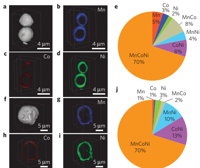
Figure 1 | Elemental mapping and association calculation using transmission X-ray tomography. a–d , 3D elemental distribution of selected NMC particles collected directly after spray pyrolysis ( a–d ) and after subsequent annealing at 850 °C ( f–i ). Single-energy tomography provides the 3D morphology of the particles ( a, f ), multi-energy tomography data with elemental sensitivity, visualized by slicing through the centre of the particles, with blue, red and green representing Mn, Co and Ni, respectively ( b–d, g–i ), and the relative concentrations of 3D elemental associations calculated by using absorption correlation tomography ( e, j ) for NMC particles collected directly after spray pyrolysis ( a–d ) and after subsequent annealing at 850 °C ( f–i ). Movies of 3D elemental distributions are shown in Supplementary Videos 1 and 2.
