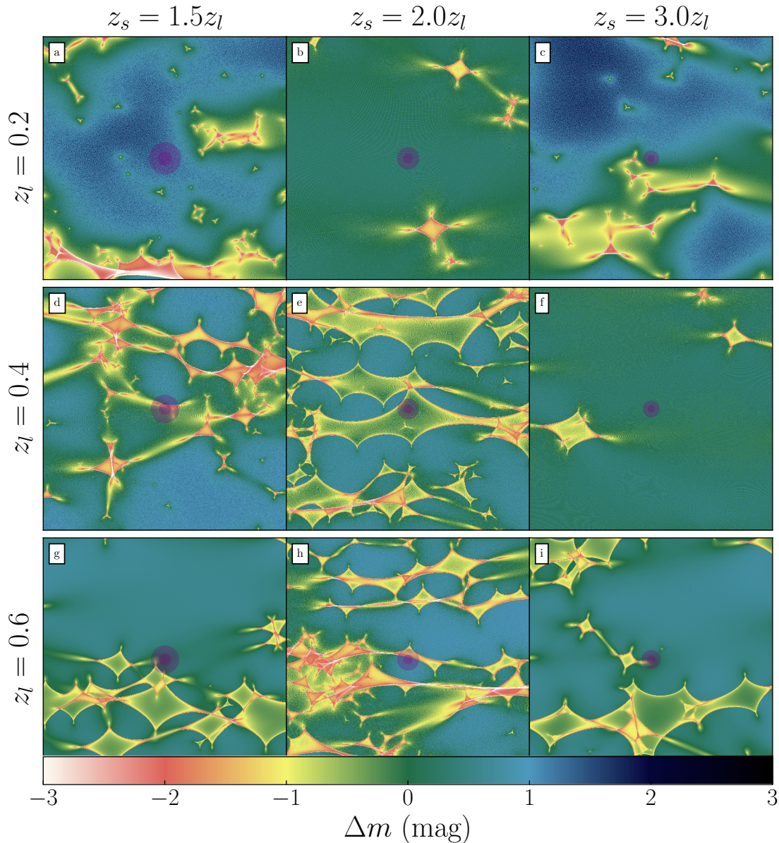
Figure 1. Source-plane magnification patterns of nine of 78,184 the lens galaxy star fields considered in this analysis. Each panel consists of 1,000^2 pixels and has a side length of 10 times the Einstein radius of a 1M_{\odot} deflector projected onto the source plane. The detailed parameters of each map are given in Table 1. The size of the exterior shell ( 4 \times 10^4 \text{ km s}^{-1} ) of the SN Ia model W7 at 20 (50) days after explosion is plotted as the interior (exterior) purple circle at the center of each map. Negative (positive) \Delta m indicates magnification (demagnification) over the theoretical average.
