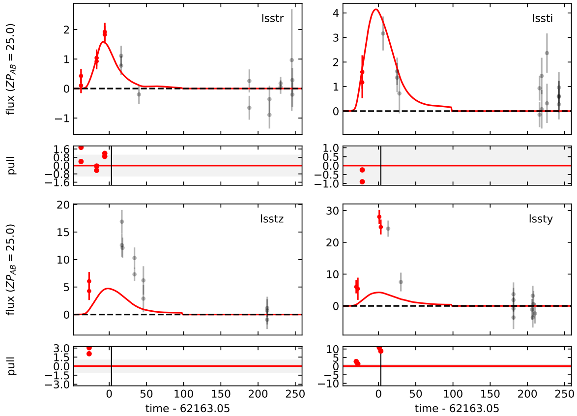
Figure 7. Detecting a z_s = 1.91, z_l = 0.96 LSST LSN Ia with SALT2. The red data points show the “current” light curve, and the red line shows the best fit SALT2 model fixed to the photometric redshift of the lens galaxy. The gray points show future observations that are not included in this iteration of the fit. The black vertical line in the residual plots shows the date when the supernova is detected. Although the model fits the data well in the bluer bands, the high redshift of the source makes the data much brighter in the infrared than the model expects given the redshift of the lens. Thus the object is detected shortly after peak due to 10\sigma discrepant points in y -band.
