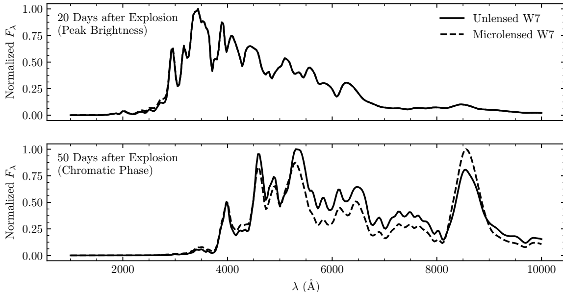
Figure 3. Rest-frame spectra of model W7 (Nomoto et al. 1984) computed with SEDONA near peak brightness and well into the onset of the infrared secondary maximum. All spectra are rescaled so that \max(F_\lambda) = 1 . The solid curve is unlensed and the dashed curve is lensed by star field (h) from Figure 1. Near peak brightness, microlensing does not have a large effect on the shape of the spectrum or the relative strengths of its features. During the chromatic phase, lensing-induced continuum shifts and spectral line distortions are visible. Such chromatic distortions can affect the colors of the supernova.
