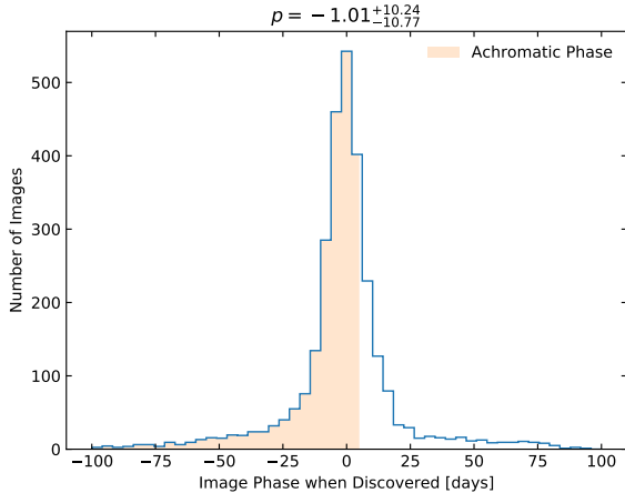
Figure 8. Phases of detected LSN images when they are discovered. 73% of the images are discovered during the achromatic phase.
