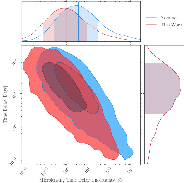
Figure 11. Joint distribution of the true time delay and the microlensing time delay uncertainty as a percentage of the true time delay for all discovered pairs of LSN Ia images. The median time delay uncertainty is 4% for light curves, but just 1% for color curve measurements in the achromatic phase. The median time delay that LSST will detect is 10 days. Marginal shaded regions show 1\sigma . Contours show 1 and 2\sigma .
