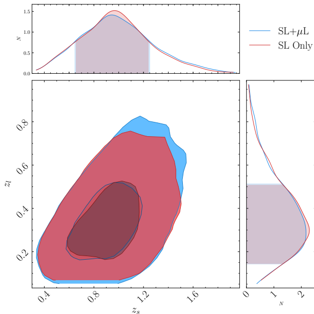
Figure 9. Source and lens redshift distributions of the LSNe Ia with at least 4 data points with S/N > 5 detected with (blue) and without microlensing (red). The joint contours show 1 and 2\sigma . The marginal shaded regions show 1\sigma .
