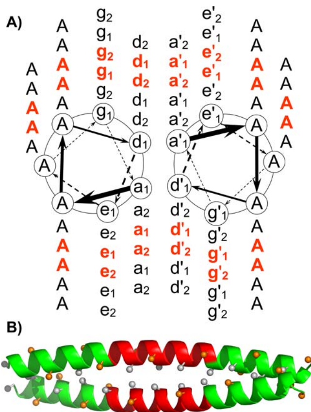
Figure 3. The Unit Cell Used for Modeling Coiled-Coil Interactions
