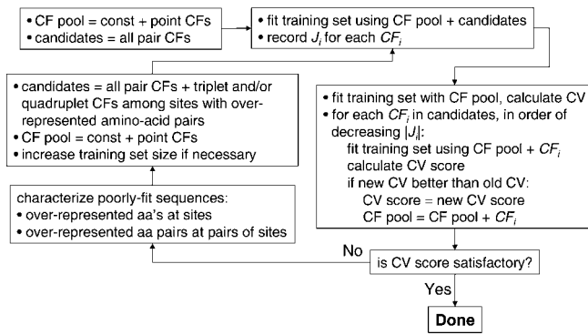
Figure 1. The Procedure for Fitting a Cluster Expansion
