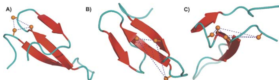
Figure 9. Important Higher-Order Clusters for the Expansion of WW-Domain Energies
