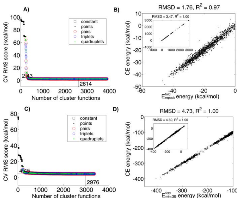
Figure 8. Cluster Expansion of WW-Domain Energies
