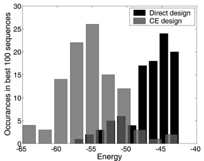
Figure 10. Distribution of the Energies of the Top 100 Sequences from Direct Design and CE Design
