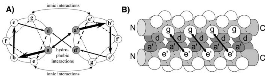
Figure 2. Schematic of a Parallel Dimeric Coiled Coil
