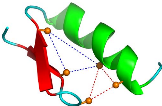
Figure 7. Important Triplet Clusters for the Expansion of Zinc-Finger Energies
