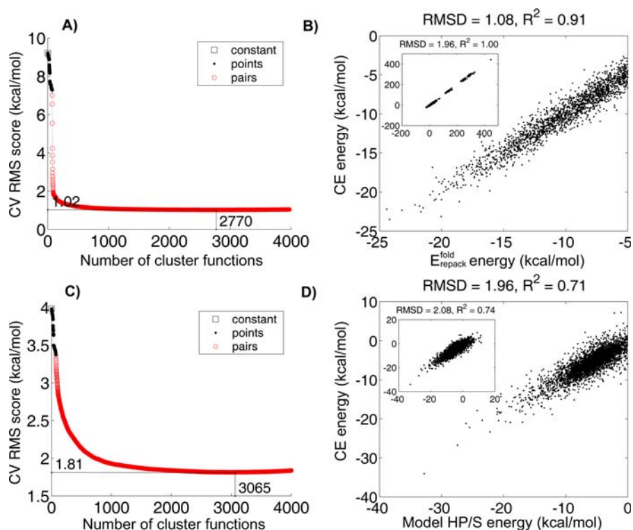
Figure 4. Cluster Expansion of Coiled-Coil Energies
