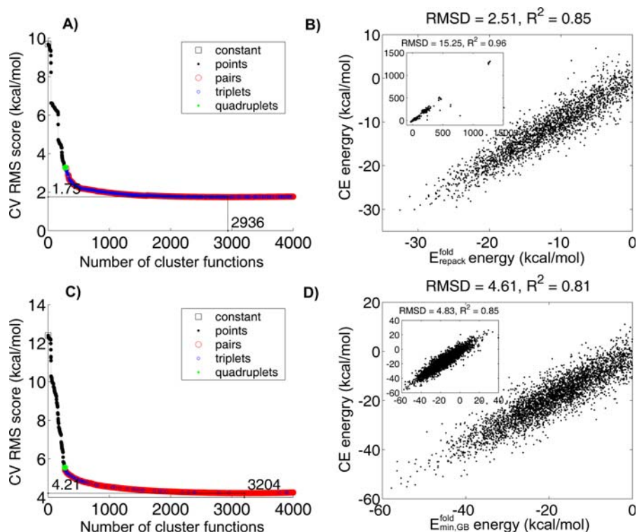
Figure 6. Cluster Expansion of Zinc-Finger Energies
