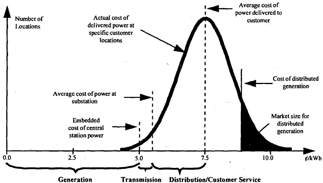
Figure 7: Potential Market for Distributed Generation
