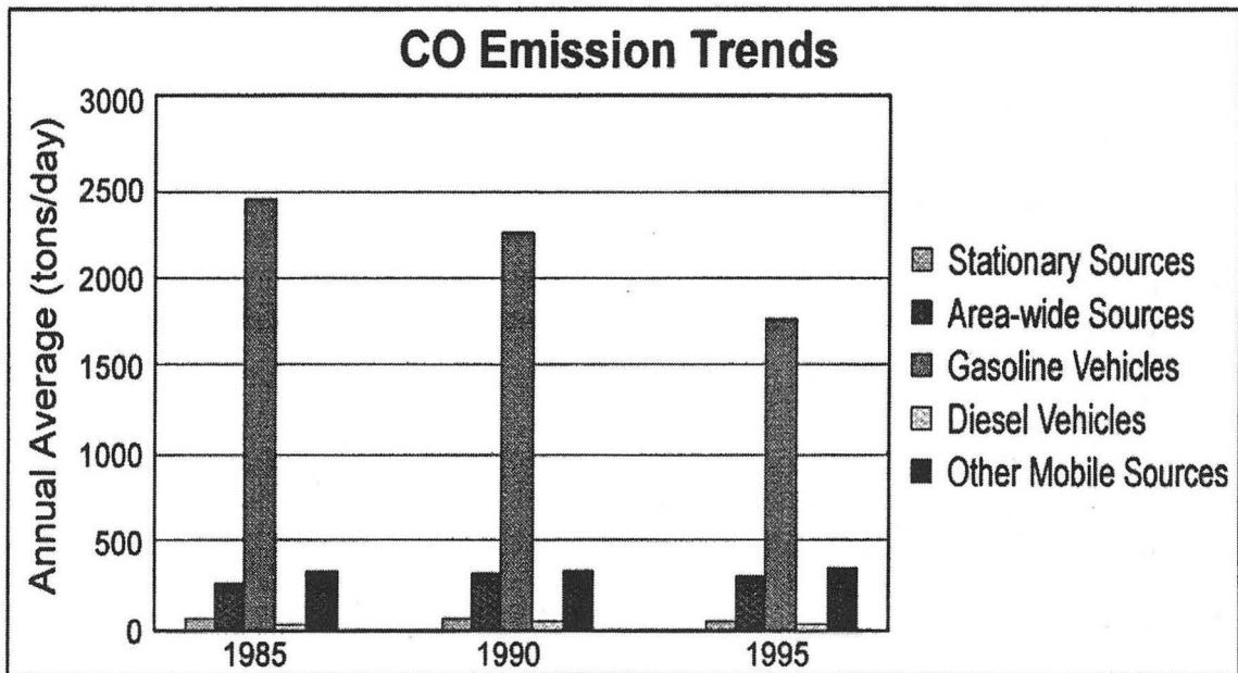
Figure 25: CO Emissions Trends
