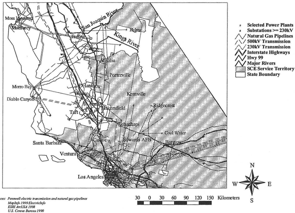
Figure 27: Electric and Gas Transmission Lines in a Sample California Neighborhood. Electric Transmission Lines 230 kV and Greater are Shown.
