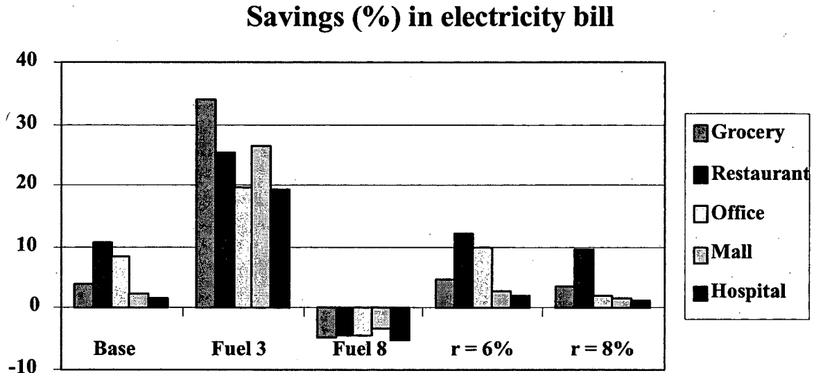
Figure 6: Customer’s Savings in Electricity Bill
