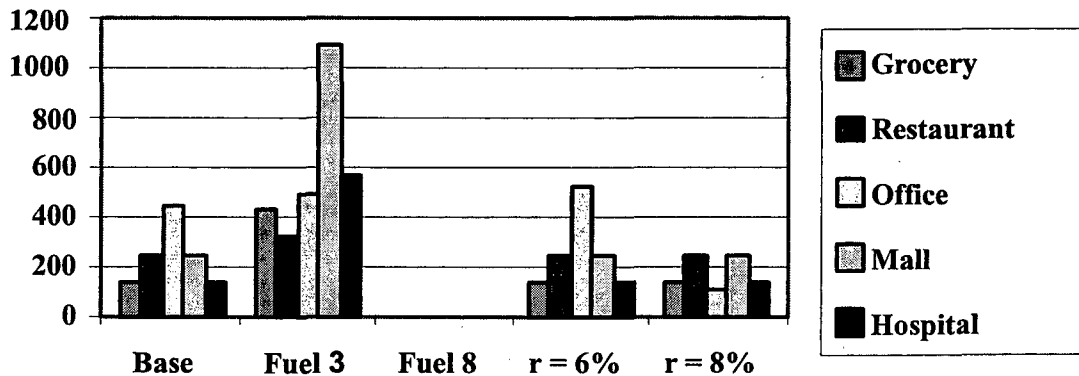
Figure 5: Distributed Generation Capacity Installed for Various Customers
