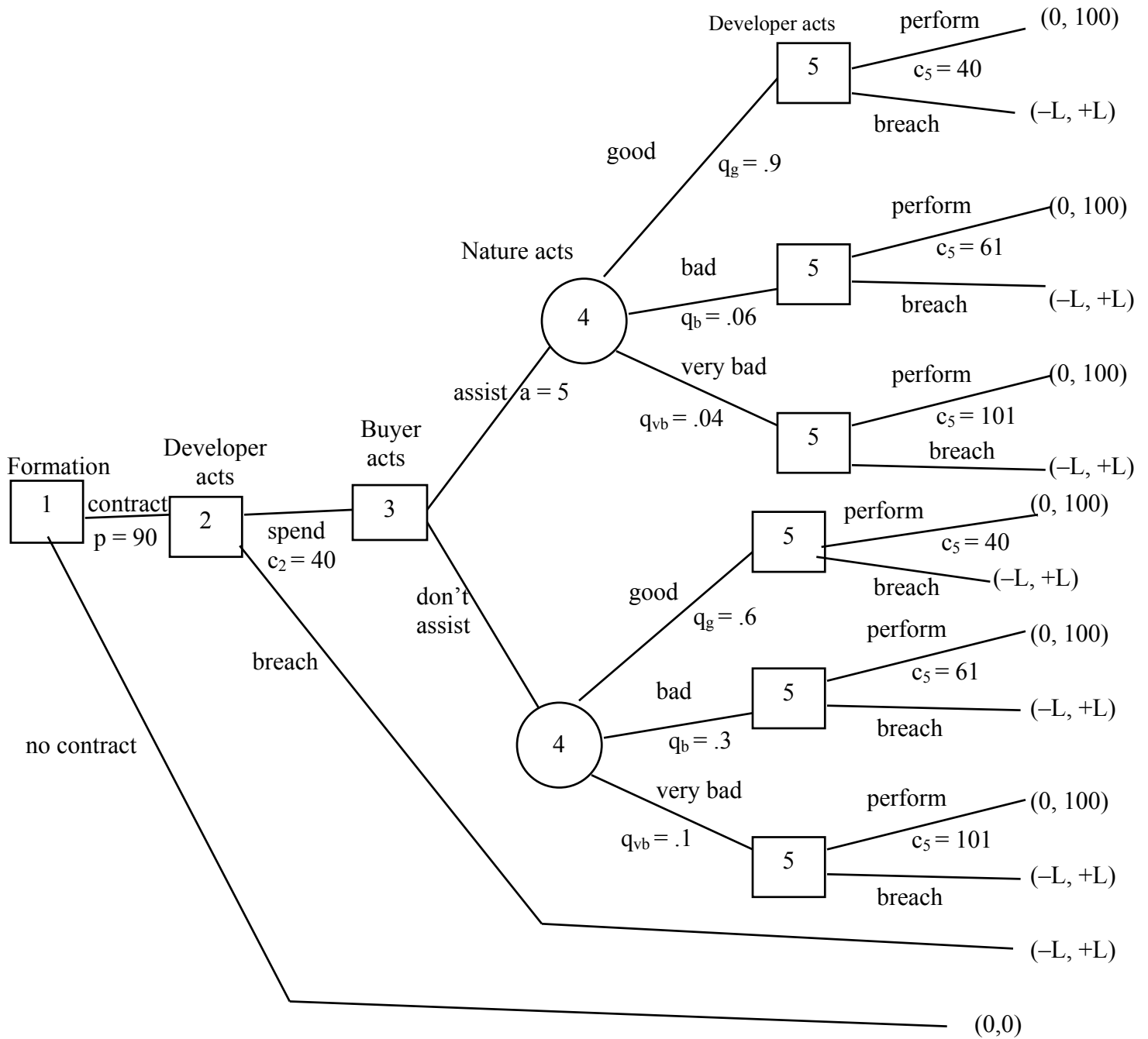
Figure 6: Example 8 as a Tree
