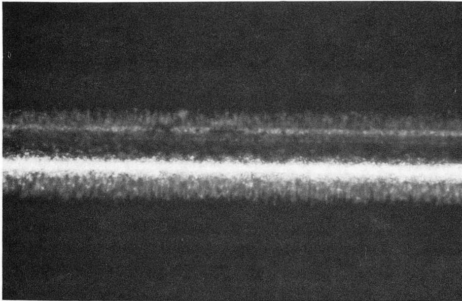
Fig. 3. Anode wire after exposure to 0.5 Coulombs charge, resulting in "bottle-brush" structure. Gas is Ar (50) + ethane (50), wire is gold-plate tungsten, and gain is high (nearly into streamer region): \sim 2 \mu\text{A} . CBB 864-2624
