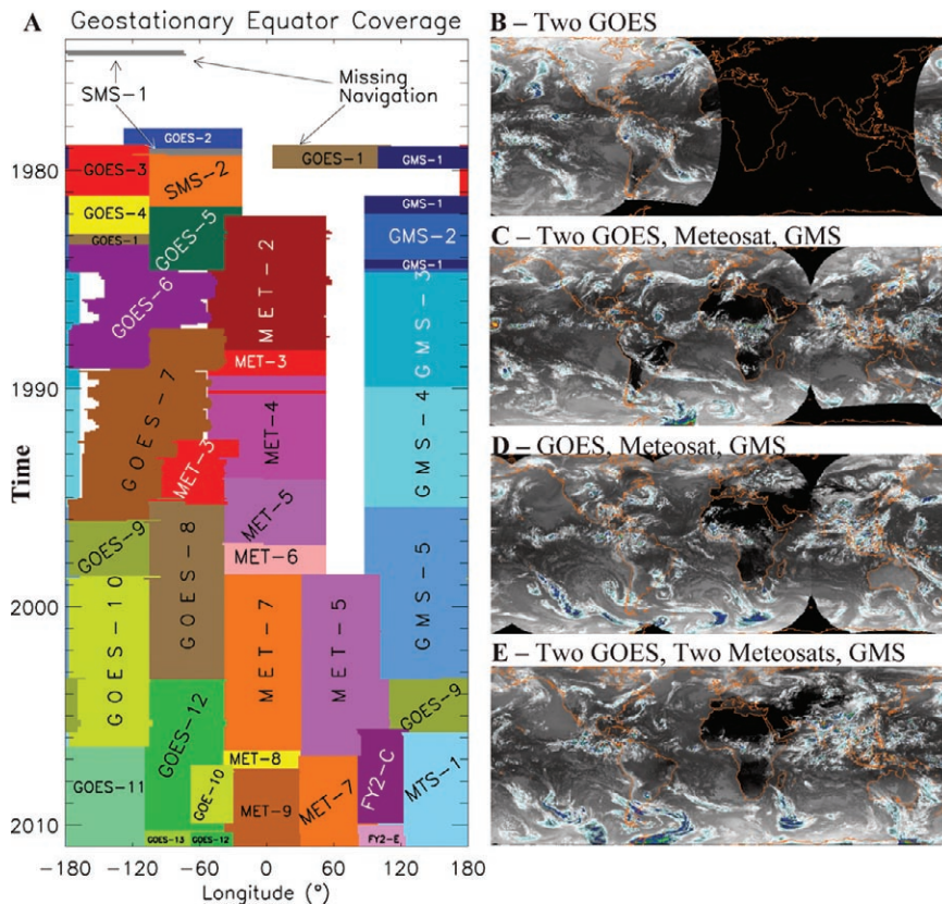
FIG. 1. (a) Time series of ISCCP B1 geostationary satellite coverage at the equator (limited to a view zenith angle of 60^\circ for illustrative purposes). (b)–(e) Sample GridSat coverage for typical satellite coverages: (b) two-satellite coverage with only GOES-East and -West in 1980, (c) four-satellite coverage that is typical of most of the period 1982–98, (d) typical three-satellite coverage when the United States was operating only one satellite (e.g., 1985–87 or 1989–92), and (e) five-satellite coverage that is typical of the current era (1998–present).
