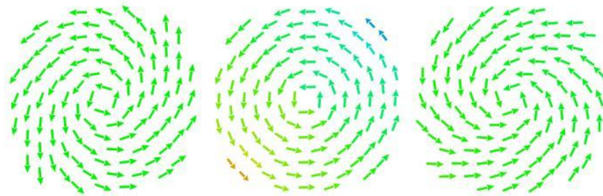
Fig. 12. (Color online) In the saw-tooth mode, which has no nodal line, spins around a ring perform an in-phase oscillation in the plane of the dot.
