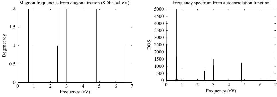
Fig. 3. Magnon spectra of a 12 spin dot with J = 1 eV (ferromagnetic) obtained by diagonalization (left) and Fourier transform of the spin autocorrelation function (right).
