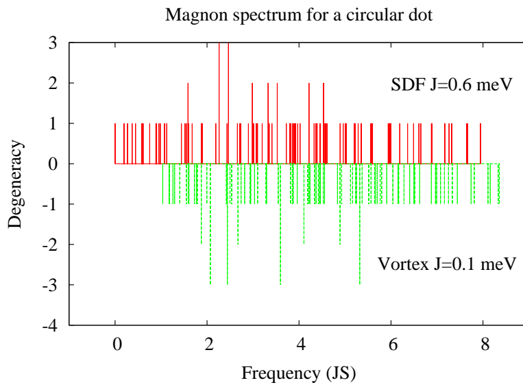
Fig. 2. (Color online) Magnon spectra of a 96 spin dot with J = 0.6 meV (ferromagnetic) and with J = 0.1 meV (vortex) above and below the x axis respectively. To have them on the same scale, frequencies are plotted in units of JS .
