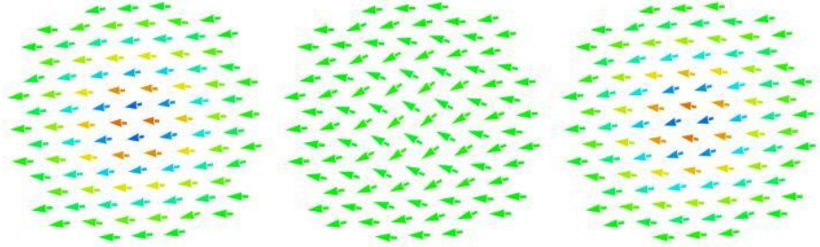
Fig. 9. (Color online) Highest-frequency HSDF mode. This state has a s-wave symmetry, but with neighboring spins oscillating out of phase. Blue spins are toward the plane (negative z -component), green spins are in the plane and red spins away from the plane (positive z -component).
