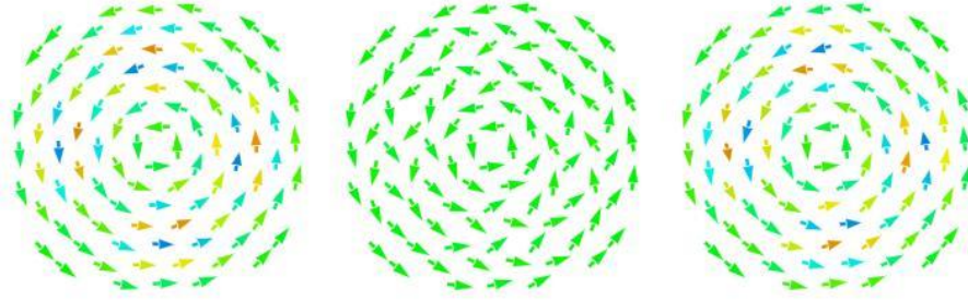
Fig. 16. (Color online) Second highest-frequency vortex mode. This mode has a d-wave symmetry.
