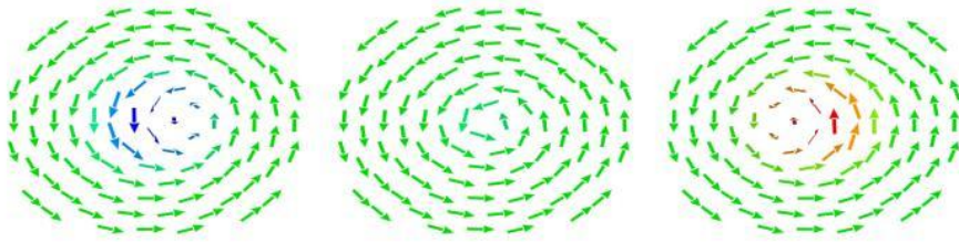
Fig. 11. (Color online) Softest mode in vortex phase near the critical point ( J = 0.25 meV). The plane of the disk has been tilted in order to show the out of plane component of the core spins. One can identify an oscillation of the out of plane component of the core spins.
