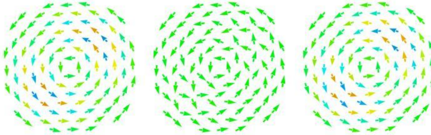
Fig. 15. (Color online) Highest-frequency vortex mode. Due to the presence of a core, the highest state has a p-wave symmetry. Blue spins are toward the plane (negative z-component), green spins are in the plane and red spins, pointing away from the plane (positive z-component).
