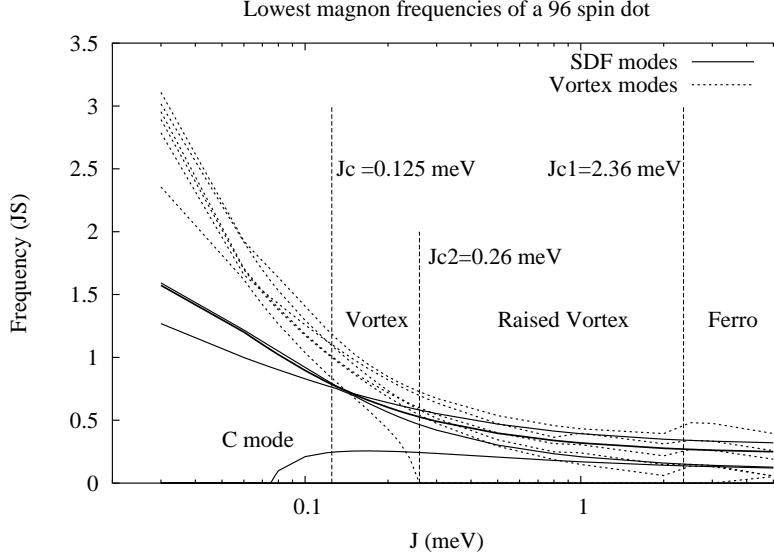
Fig. 7. Lowest magnon frequencies as a function of the exchange coupling near the transition point in both phases for a 96-spin dot. The critical J where the total energies of these phases become equal is also shown ( J_c = 0.125 meV). Magnon instability of each phase, however, occurs at a further point ( J_{c3} = 0.075 meV : C-mode instability of HSDF, J_{c2} = 0.26 meV : vortex raising, and J_{c1} = 2.36 meV : spontaneous crossover to HSDF). In principle, as the system size is finite, the crossover to the raised vortex phase can take place after a finite time for any J between J_c (=0.125) and J_{c1} (=2.36 meV), see also Fig. 8.
