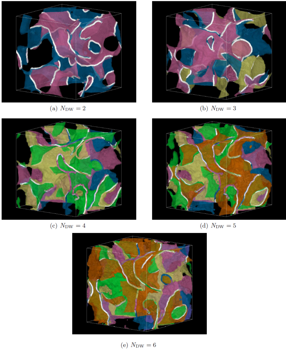
Figure 1.13: This graph is cited from [9]. The white lines correspond to the position of the core of strings, which is identified by using the method described in Appendix B.1 of [10]. N_{DW} domain walls are represented by surfaces with various colors, which are identified by using the method described in Appendix B.2 of [10].
