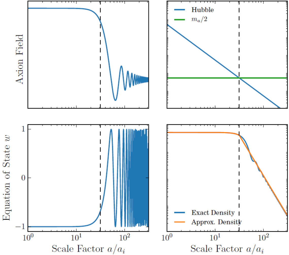
Figure 1.5: This shows Eq.(1.164) with p = 1/2 . This is from Figure 4 of [5]. Vertical dashed lines show the condition defining A \equiv m_a/H(R_{\text{osc}}) \equiv 2 as condition in Eq.(1.162) and Eq.(1.163), also used the approximation \rho_a(R) = \rho_a(R_{\text{osc}})(R_{\text{osc}}/R)^3 when (R > R_{\text{osc}}) as well as \rho_a(R_{\text{osc}}) \simeq m_a^2 a_i^2/2 , hence the axion energy density is controlled by initial conditions. The right-down shows a comparison of A = 2 and is fully numerical. On the other hand, if we consider A = 3 the result can be fit very well as A = 2 did. The important things are (1) upper-left, the axion field frozen when m_a is in of scale-regime ( H > m_a , see upper-right). (2) lower-right, the axion energy density decays shortly once enters to scale regime.
