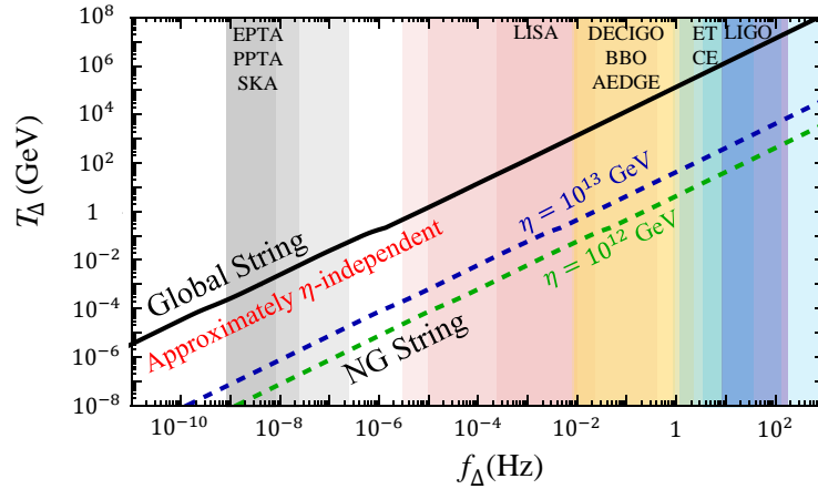
Figure 4.6: Frequency f_{\Delta} where the GW spectrum from cosmic strings would be altered due to a transition to a non-standard cosmology at T_{\Delta} (Eq.(4.32)): the comparison between the results for global strings (the upper-left black line) and NG strings [13, 14] (the lower-right dashed lines). The relevant experimental sensitivities are also shown in different colors, where the darkest bands indicate peak sensitivities. This illustrated the f_{\Delta} - T_{\Delta} relation given in the main text.
