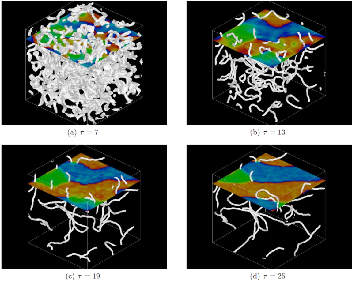
Figure 1.14: This graph is cited from [9]. The value of \theta_a varies from -\pi (blue) to \pi (red). At late times, the value of \theta_a is separated into three domains represented by blue, red, and green regions. Domain walls are located around the boundary of these three regions, \theta_a = \pi/3 , \theta_a = -\pi/3 , and \theta = \pm\pi . Strings, which are represented by white lines, pass through the point where three regions meet each other.
