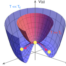
Figure 1.4: The PQ complex scalar potential with PQ symmetry breaking, the figure is cited from [4].
