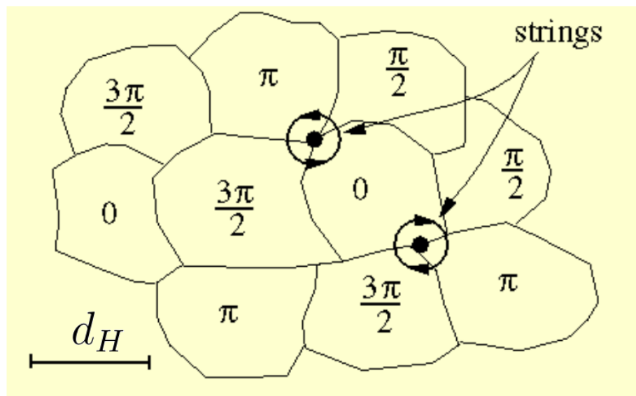
The Kibble mechanism for the formation of cosmic strings.
