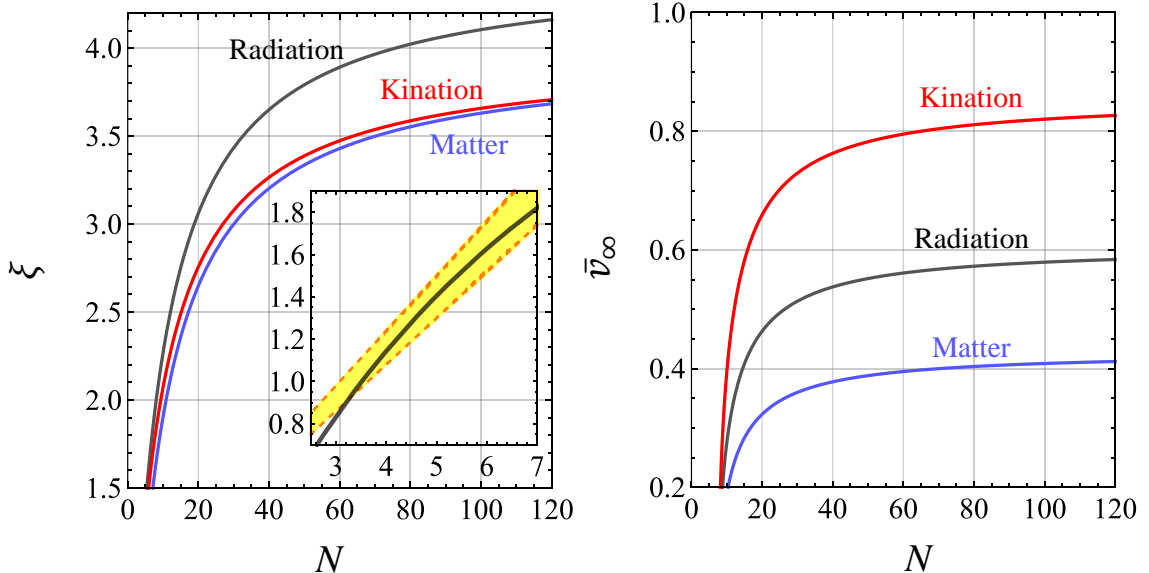
Figure 4.1: The number of global string per Hubble volume \xi and the average long string velocity \bar{v}_\infty as functions of N \equiv \ln \frac{L}{\sigma} , as predicted by the VOS model, for different background cosmologies. The subfigure in the left panel is the zoom-in of \xi evolution in the low N range during radiation domination, where the yellow band shows the 1\text{-}\sigma uncertainty region based on the finding by simulation (as shown in Eq.(4.9) with \beta \sim 0.20 ).
