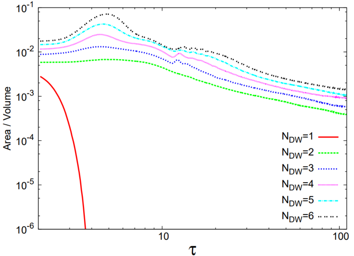
Figure 1.12: This graph is cited from [9] shows the area of domain walls with different domain wall numbers N_{DW} . The \tau is conformal time. As we see in Fig.1.8, the domain wall will decay very fast at N_{DW} = 1 case. On the other hand, domain walls will decay very slowly with N_{DW} > 1 , therefore, eventually, a non-neglectable domain wall density will dominate in the universe, the so-called Axion Domain Wall Problem.
