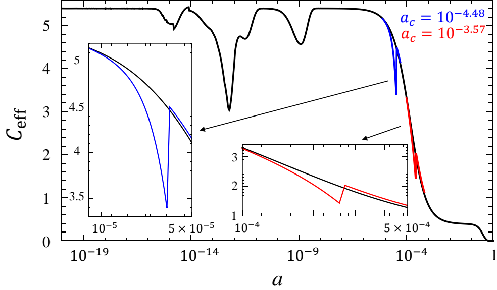
Figure 5.4: C_{\text{eff}} versus scaling factor a . The black curve is in \Lambda\text{CDM} . The modified universes with the EDE are shown as a_c = 10^{-4.48} and a_c = 10^{-3.57} as blue and red, respectively.
