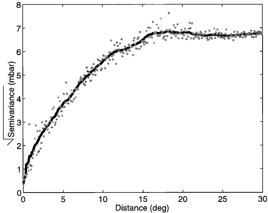
Figure 10. Square root of the semivariance of pressure measurements for the United States in 0.1^\circ bins (shaded dots) and smoothed (solid line).
