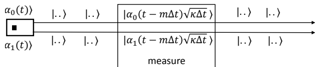
FIG. 3: Illustration of the “history tail” idea. Since the qubit does not evolve by itself, we can think in terms of superposition [Eq. (46)] of two evolutions of the resonator state [ |\alpha_0(t)\rangle and |\alpha_1(t)\rangle ], which leave the “history record” in the form of propagating field, leaked from the resonator. We call this propagating field a “history tail”. The quantum Bayesian formalism developed in this paper is based on measuring small pieces of the history tail in the textbook way. The corresponding state collapse leads to change of the coefficients in the superposition, which is the evolution due to measurement.
