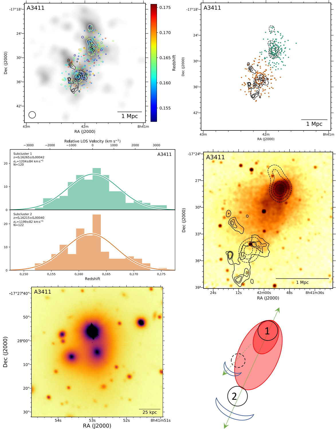
Figure 26. Top left: DS-test over red sequence Subaru/SuprimeCam r-band luminosity distribution with linearly spaced white contours. The black contours show GMRT 325 MHz contours (van Weeren et al. 2017). Top right: Subcluster membership of spectroscopic cluster members assigned with our GMM analysis. The same GMRT contours (solid) and red sequence luminosity contours (dashed) are depicted. Middle left: Subcluster redshift histogram with colors matching the image at the top right. Middle right: 215 ks Chandra image with the same GMRT radio contours (solid) and red sequence luminosity contours (dashed). Bottom left: 150 kpc cutout of the Subaru r-band image centered on the cluster BCG in subcluster 1. Bottom right: Preferred merger scenario. A3411 is composed of at least two subclusters, where the northern subcluster 1 is A3411 and the southern 2 is A3412. Subcluster 1 is associated with a cool-core remnant and wake feature indicating the ICM is traveling northward. The two subclusters have very similar velocity dispersions and redshifts suggesting a 1:1 mass ratio merger in the plane of the sky. There is evidence of composite structure in subcluster 2 as presented in van Weeren et al. (2017), where a small subcluster has created a shock that reaccelerated particles associated with an AGN.
