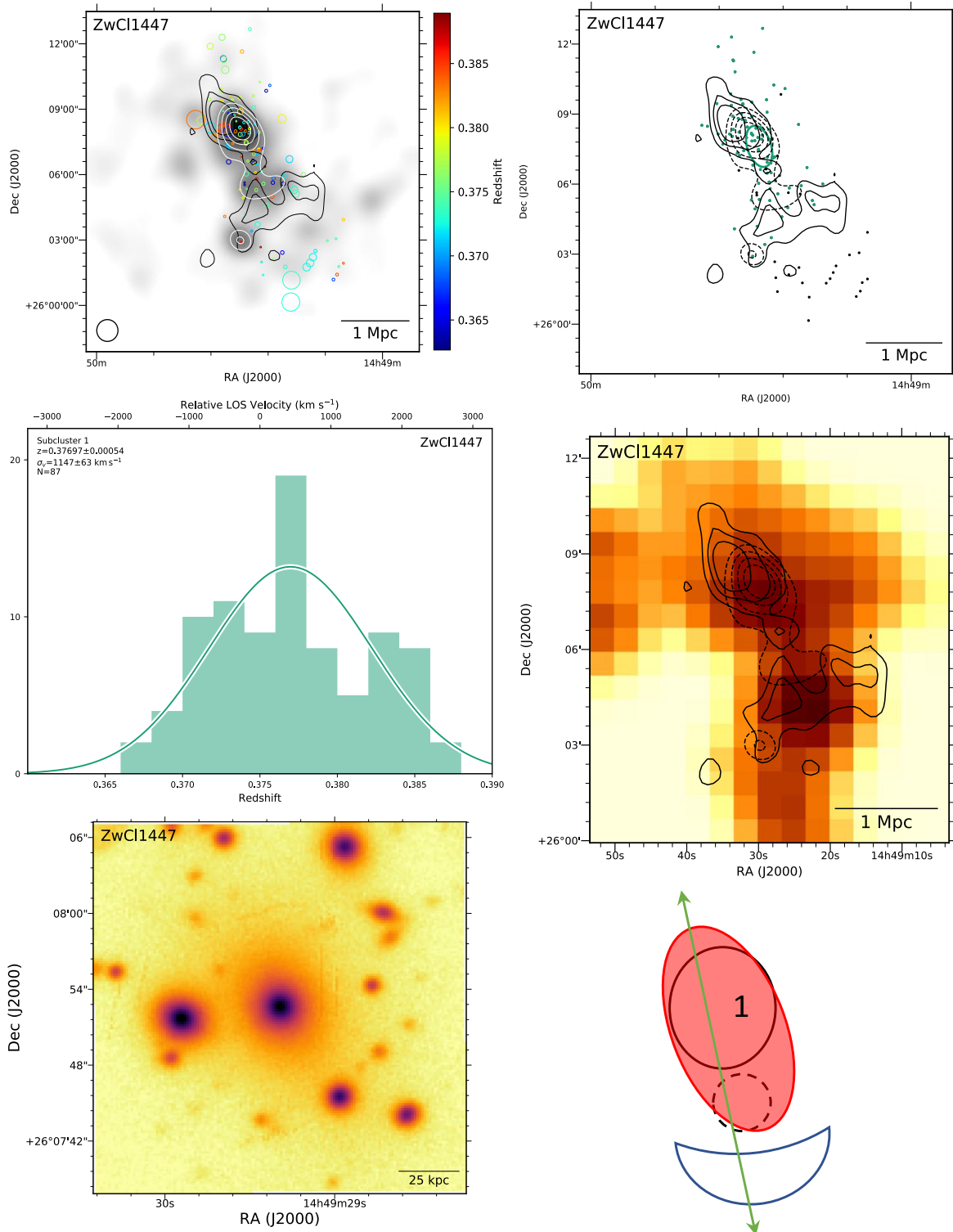
Figure 35. Top left: DS-test over red sequence Subaru/SuprimeCam r-band luminosity distribution with linearly spaced white contours. The black contours show VLA 1.4 GHz contours (Govoni et al. 2012). Top right: Subcluster membership of spectroscopic cluster members assigned with our GMM analysis. The same VLA contours (solid) and red sequence luminosity contours (dashed) are depicted. Middle left: Subcluster redshift histogram with colors matching the image at the top right. Middle right: 21 ks ROSAT image with the same VLA radio contours (solid) and red sequence luminosity contours (dashed). Bottom left: 150 kpc cutout of the Subaru r-band image centered on the cluster BCG. Bottom right: Preferred merger scenario. The GMM did not detect two subclusters; however, the red sequence luminosity is elongated along the same axis as the X-ray surface brightness and radio relics. We propose a north-south merger axis. Further spectroscopy in the south is necessary to better constrain the subcluster velocities.
