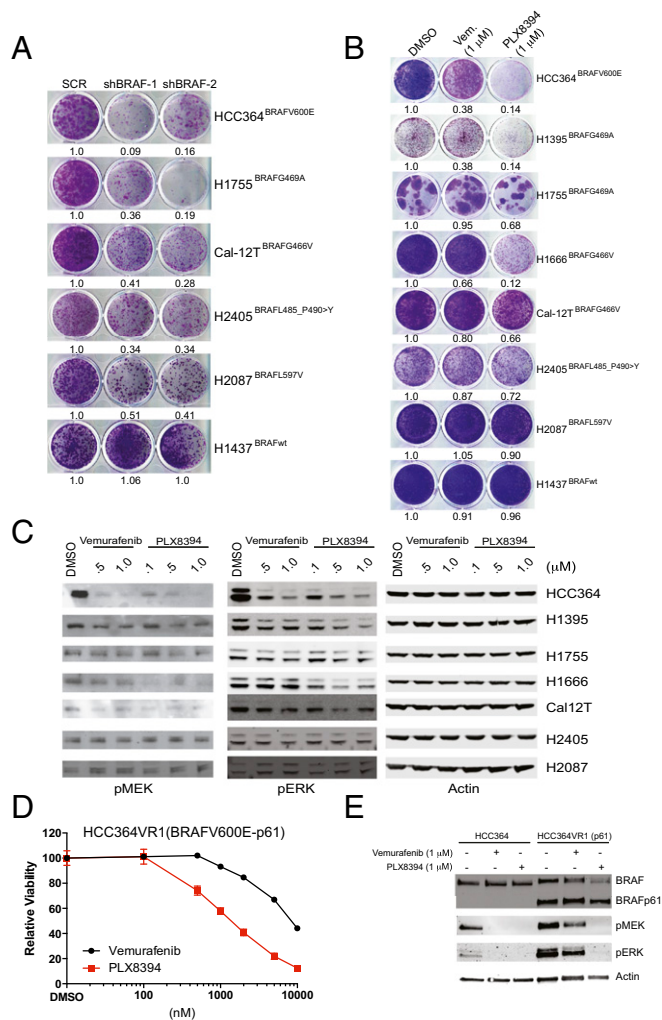
Fig. 1. The effects of PLX8394 RAF inhibitor treatment in BRAF V600E and non-V600 BRAF -mutant LA cells in vitro. ( A ) BRAF -mutant LA cell lines are addicted to each oncoprotein. Shown is the cell growth upon shRNA-mediated knockdown, conducted and analyzed as reported (4). ( B and C ) The effects of RAF inhibitor treatment with each indicated agent on growth ( B ) and signaling ( C ) in each BRAF -mutant LA cell line. The experiment was conducted and analyzed as reported (4), using the indicated drug doses. Vem, vemurafenib. ( D and E ) The effects of RAF inhibitor treatment with each indicated agent on growth ( D ) and signaling ( E ) in BRAF V600E LA cells with acquired vemurafenib resistance that express a vemurafenib-insensitive, truncated form of BRAF V600E . The experiment was conducted and analyzed as reported (4), using the indicated drug doses. All data shown represent three independent experiments, mean ± SEM, P < 0.01 .
