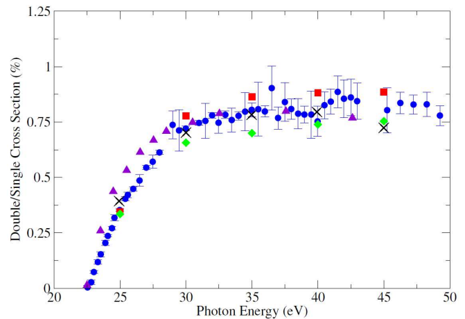
FIG. 2: (Color online) Double to single ionization cross section ratios for single photon double ionization of Mg. Black crosses: present results in the length gauge, red squares: TDCC results [10], green diamonds: RMPS results [10], violet triangles: CCC results [14], blue circles: experimental measurements [20].
