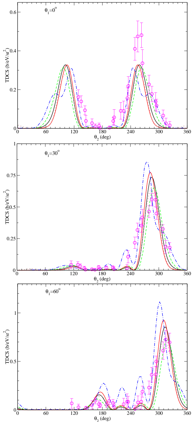
FIG. 4: (Color online) Triple differential cross section (TDCS) for DPI from magnesium at 55.49 eV photon energy for equal energy sharing. Each panel shows plots the second electron in the coplanar geometry when the first electron is fixed at the angle shown relative to the polarization. Solid (black) curve: present results in the length gauge, solid (red) curve: present results in the velocity gauge, dashed (green) curve: TDCC results [19], dotted (brown) curve: CCC non-resonant results, dashed-dot (blue) curve: CCC resonant results [18], magenta circles: experimental measurements [18]. 1 \text{ b} = 10^{-24} \text{ cm}^2 .
