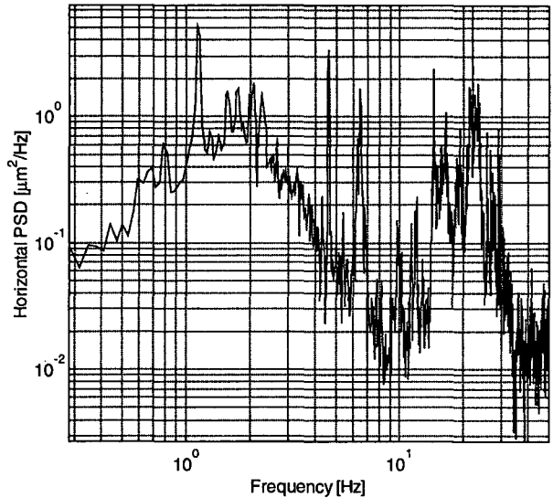
Figure 3: Power spectral density of the horizontal orbit.
