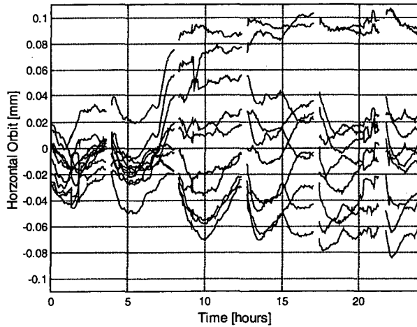
Figure 1: Horizontal orbit stability without feedback, August 15, 1998.
