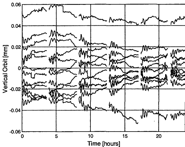
Figure 2: Vertical orbit stability without feedback, August 15, 1998.
