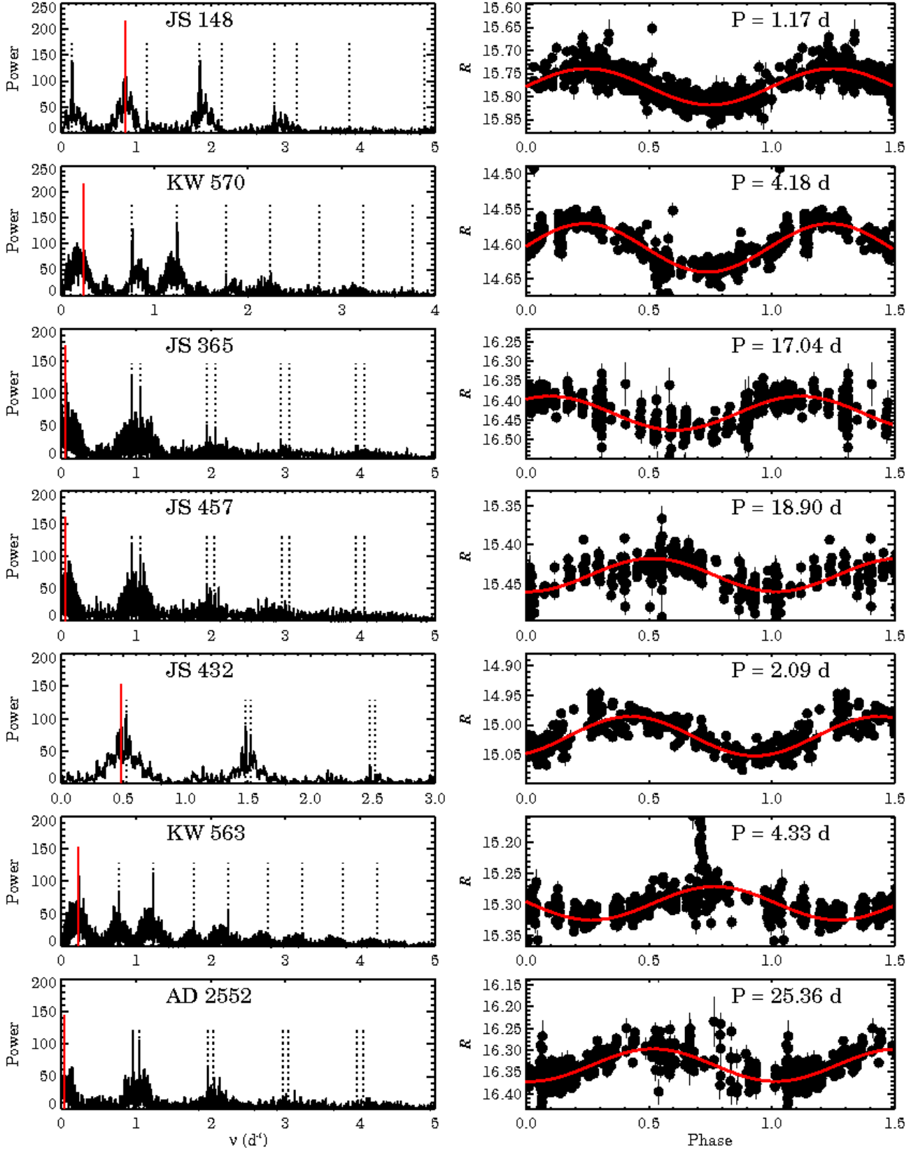
FIG. 11.— Periodograms (left column) and phased light-curves (right column) for each Praesepe member with a rotation period measured from our PTF data. The adopted P_{rot} is flagged in each periodogram with a red line; potential beat frequencies between this period and an assumed one-day alias are flagged with black dotted lines. Error bars are overlotted on each data point in the light-curve, which is phased by P_{rot} . For clarity, we show 1.5 phases of each star’s period and plot a sinusoid curve with the same amplitude and period as the variability measured for each star.
