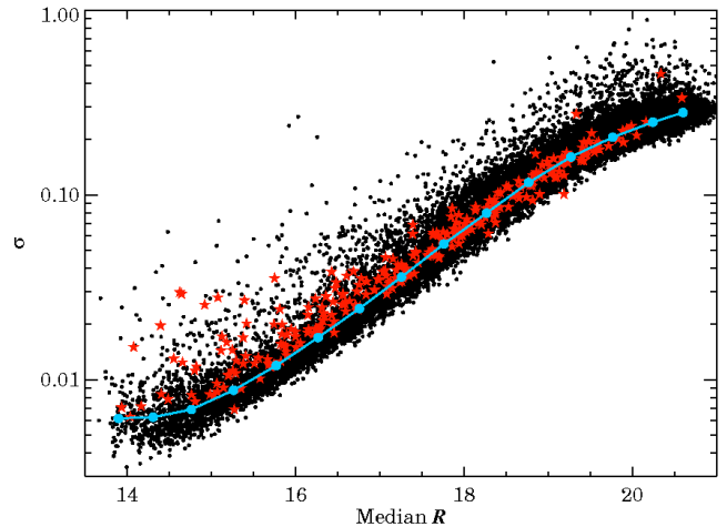
FIG. 2.— \sigma versus median R magnitude of objects detected in multiple epochs in field 110003. Praesepe members are shown as red stars; the \sim 30,500 non-members with PTF light-curves in this field are shown in black. At the bright end, the scatter in the light-curves exceeds the formal photometric errors by factors of a few, indicating that the precision is limited by systematic effects rather than by random photometric error. We plot in blue the median \sigma for non-members obtained when placing the magnitudes in bins of width 0.5 \text{ mag} (e.g., for the 1266 non-members with 16.5 \leq R < 17 \text{ mag} , the median \sigma = 0.02 \text{ mag} ). Praesepe members have systematically higher \sigma (and are thus more variable) than the median field star for R \lesssim 17 .
