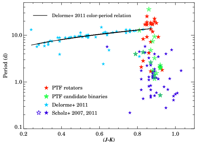
FIG. 5.— Color-period distribution for Praesepe, with the Delorme et al. (2011) color-period relation overlotted.
