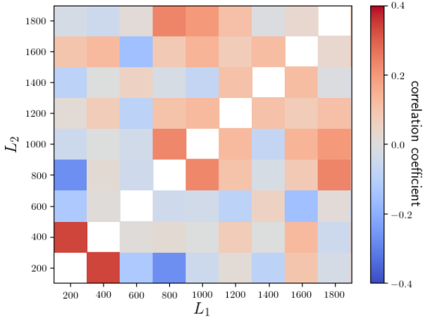
Figure 7. Correlation coefficients of the cross power spectrum between CMB lensing and cosmic shear, estimated from 100 realizations of simulations.
