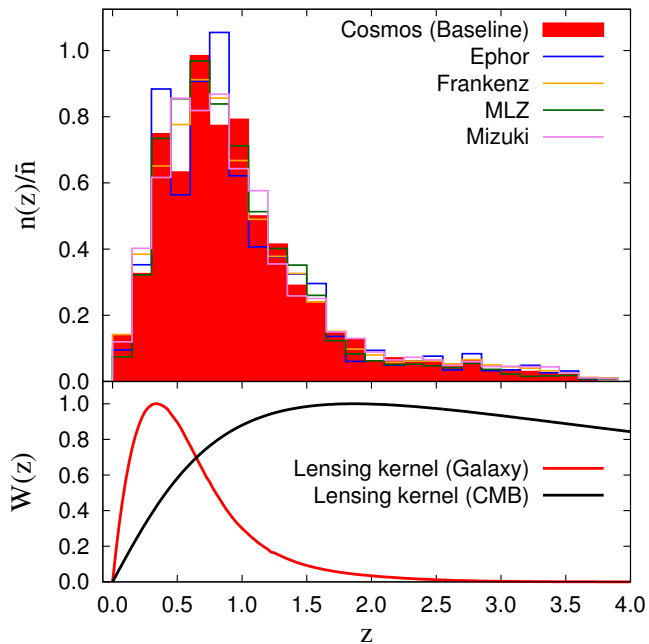
Figure 1. Top: Redshift distributions of HSC galaxies used for the cross-correlation analysis. The filled histogram shows our baseline estimate, whereas open histograms show distributions estimated from different HSC photometric redshift estimates (Tanaka et al. 2018). Bottom: Lensing kernels of the HSC galaxies (red) and CMB (black). The lensing kernels are normalized by their maximum values. We only show the galaxy lensing kernel for the baseline distribution.
