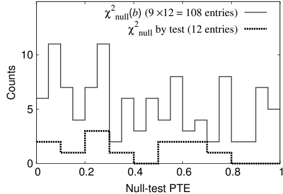
Figure 3. Null-test PTE distributions of \chi_{\text{null}}^2(b) and \chi_{\text{null}}^2 by test (dotted line). Both distributions are consistent with the expectation from the uniform distribution (see also Table 1).
