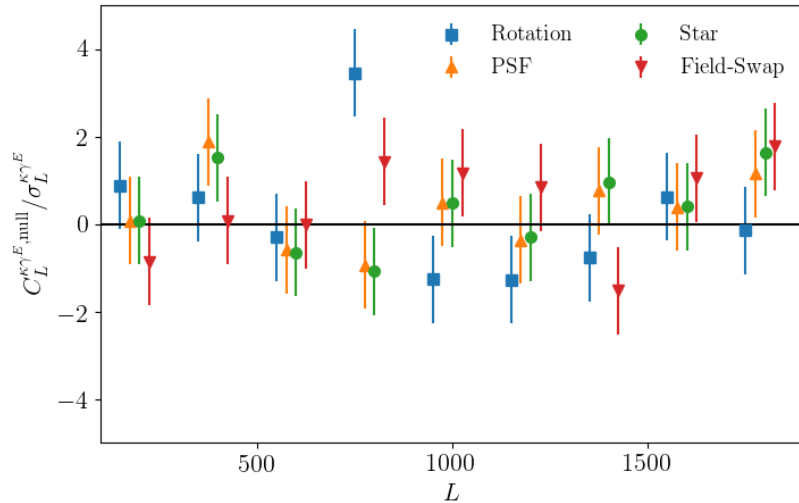
Figure 5. Cross power spectra between the HSC null test maps and the real POLARBEAR lensing map. We consider HSC null test maps derived by randomly rotating ellipticities of real HSC galaxies (“Rotation”), from star ellipticities (“Star”), from PSF ellipticities (“PSF”), which are measured in another HSC field (“Field Swap”). The cross power spectra are normalized by their statistical uncertainties.
