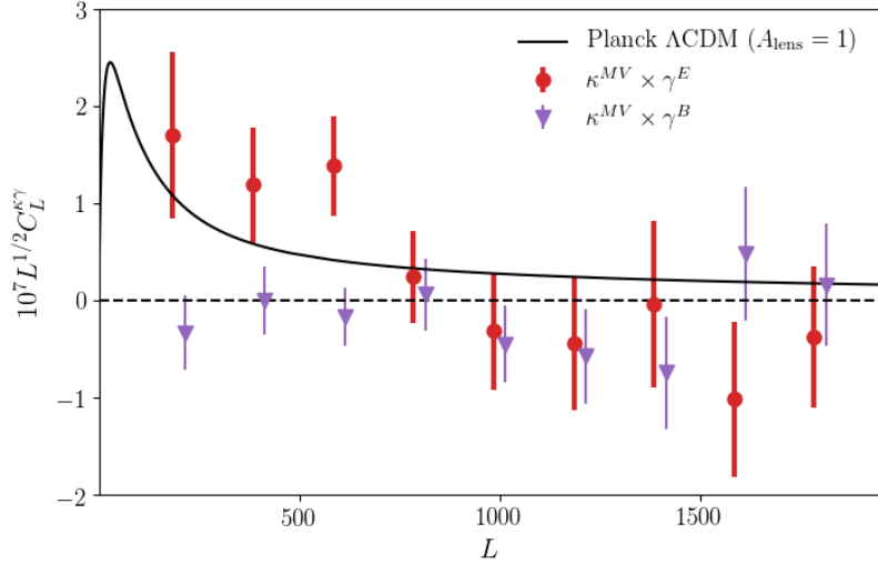
Figure 6. The cross power spectra between the CMB lensing convergence from POLARBEAR and the cosmic shear from HSC. The CMB lensing map is obtained from the optimal combination of the EE and EB estimators (MV). We show the cross spectrum between the HSC shear B -mode and the CMB lensing convergence, consistent with zero as expected. The black solid line shows the theoretical prediction, assuming the Planck 2018 best-fit cosmological parameters for the flat \Lambda CDM model.
