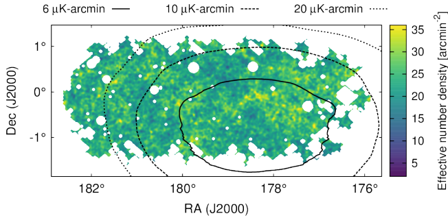
Figure 2. The overlapping sky coverage of POLARBEAR and HSC maps in this work. Contours show the noise level of the POLARBEAR CMB polarization maps. The color map shows the effective number density of the HSC galaxy catalog.
